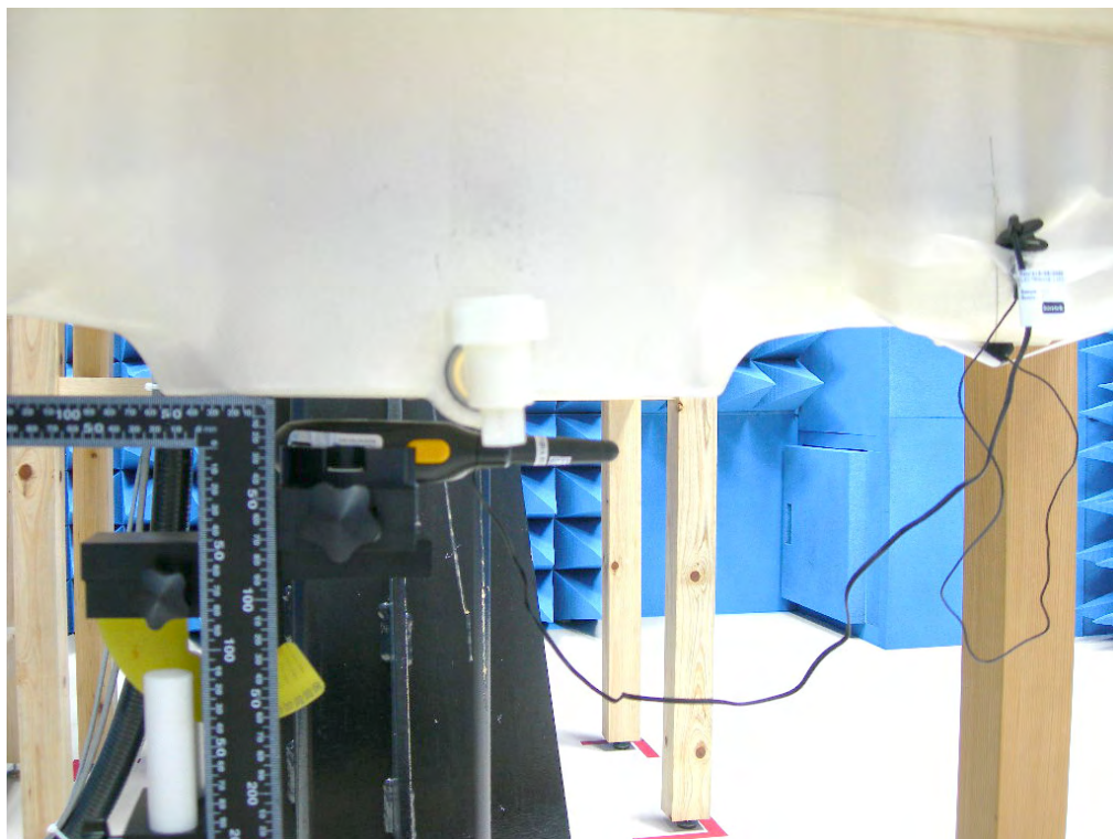
Figure 17.SAR Test Setup w/o Belt Clip
