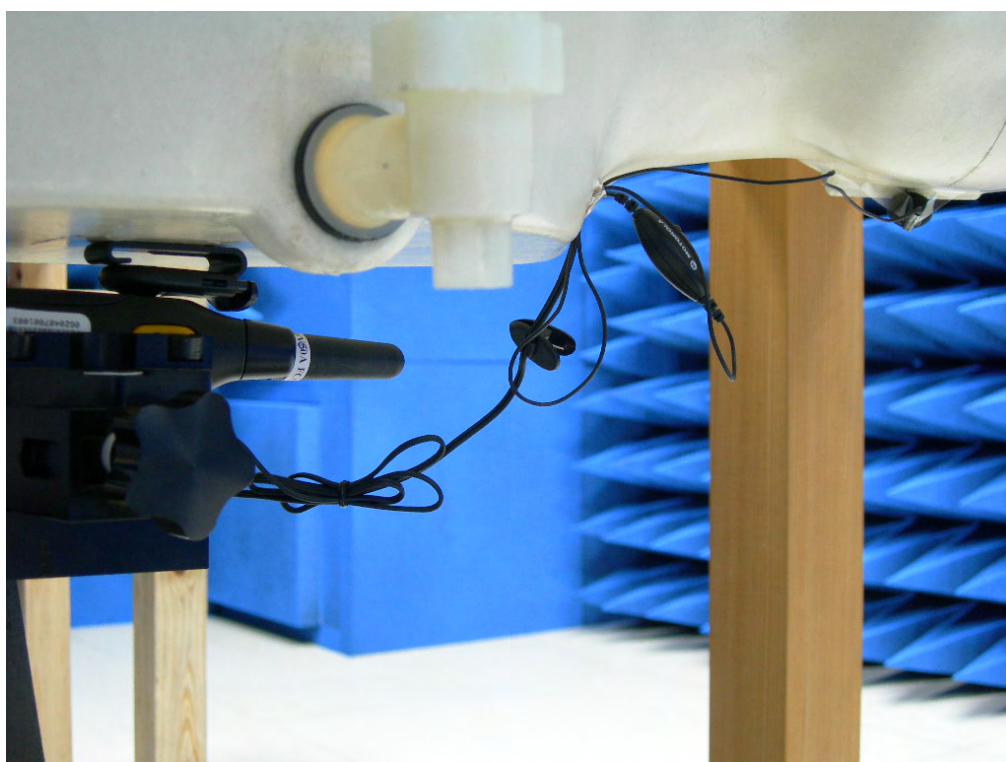
Figure 16.SAR Test Setup with Belt Clip
