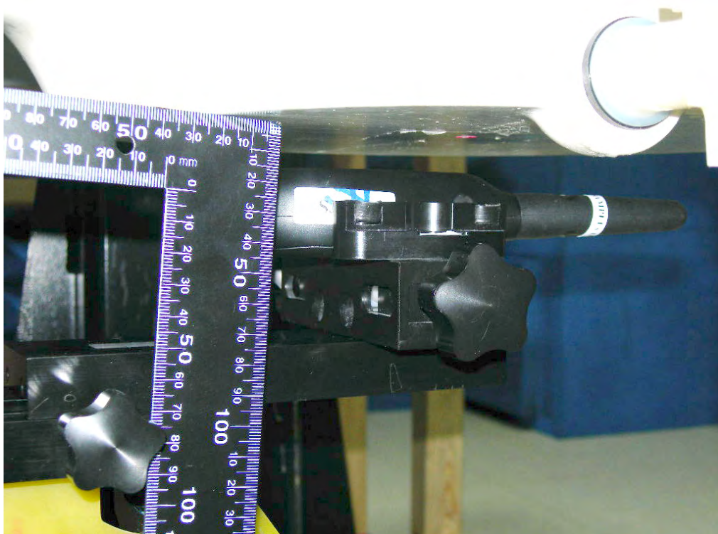
Figure 15. SAR Test Setup Face Position
