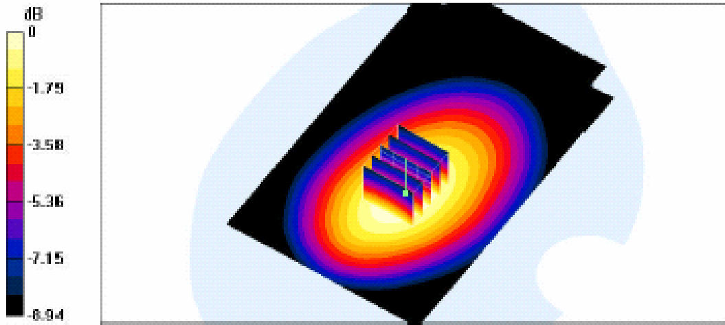
SAR Test Result for GMRS Face SAR -1.5 cm Spacing-Channel 15
