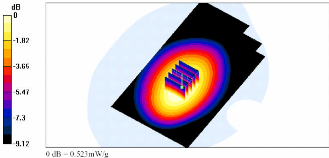
SAR Test Result for GMRS Body SAR w / Belt -clip Channel 15
