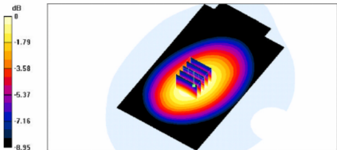
SAR Test Result for FRS Face SAR -1.5 cm Spacing-Channel 8
