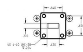
MATING FACE OF KRFU A4J4 MATING FACE OF B1 A6J3A & A6J3B (DIMENSION ARE IN INCHES)
