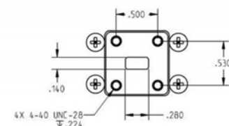
MATING FACE OF KRFU A4J3 MATING FACE OF B1 A6J4A & A6J4B (DIMENSIONS ARE IN INCHES)
