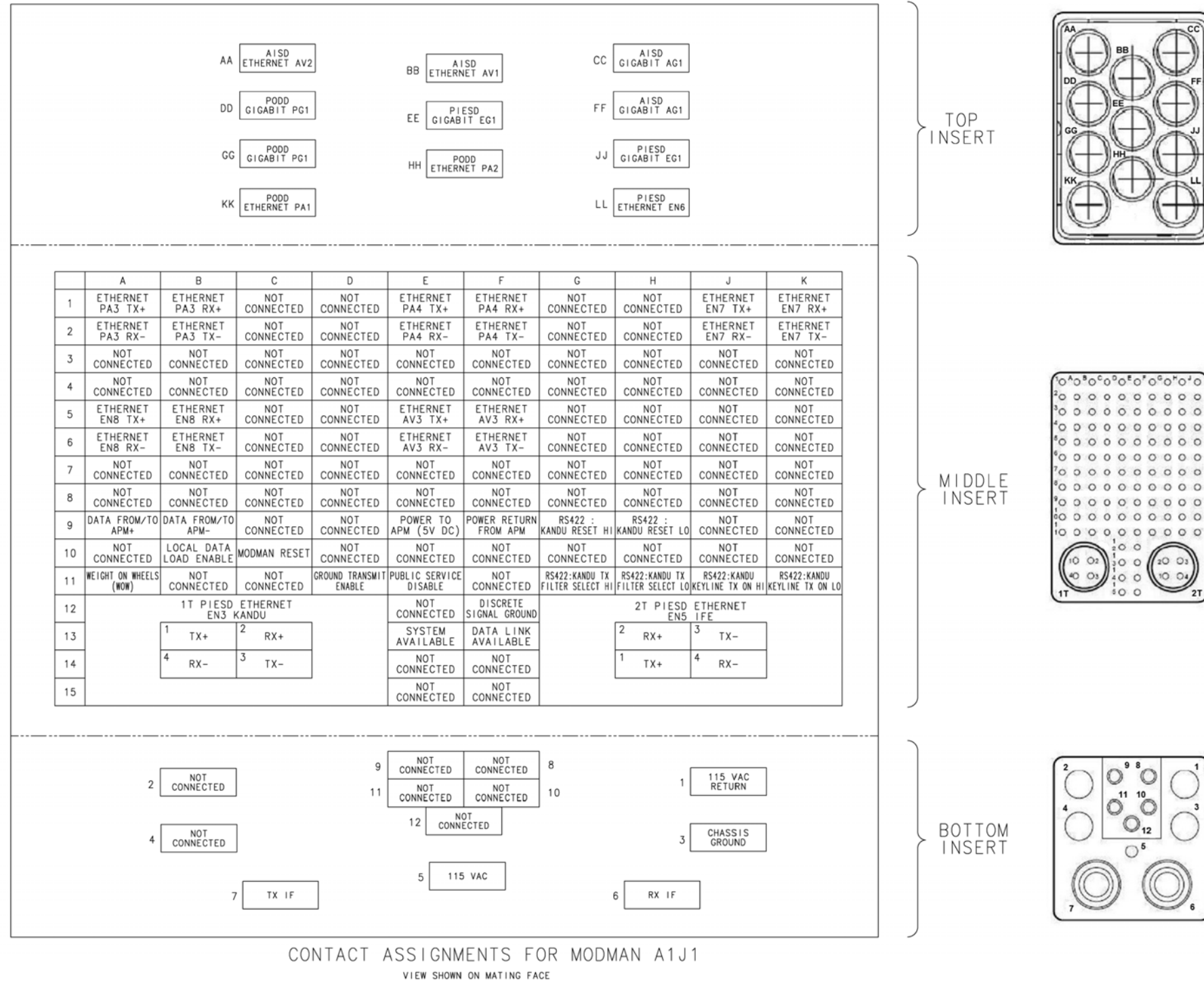
Figure 4-36. (Sheet 6 of 8) JetWave™ System Interconnect Diagram - FMA (KRFU Outside Aircraft Fuselage), (90401047-1, REV F)
