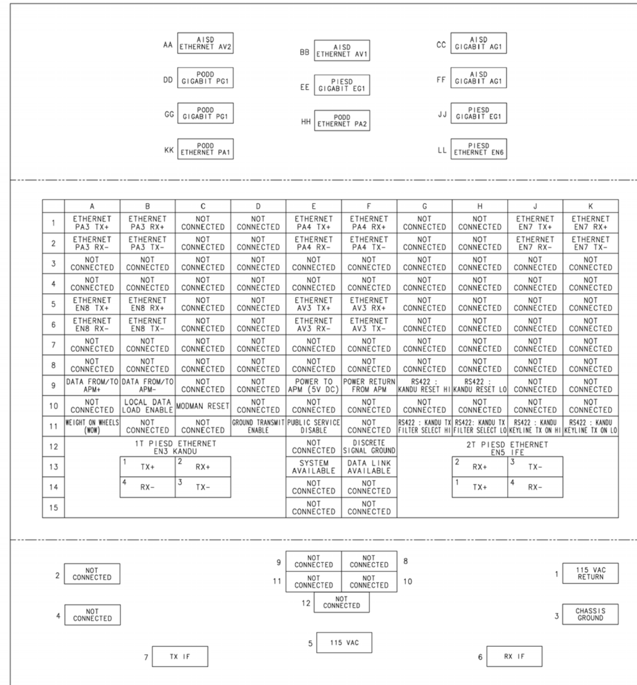
CONTACT ASSIGNMENTS FOR MODMAN A1J1 VIEW SHOWN ON MATING FACE
