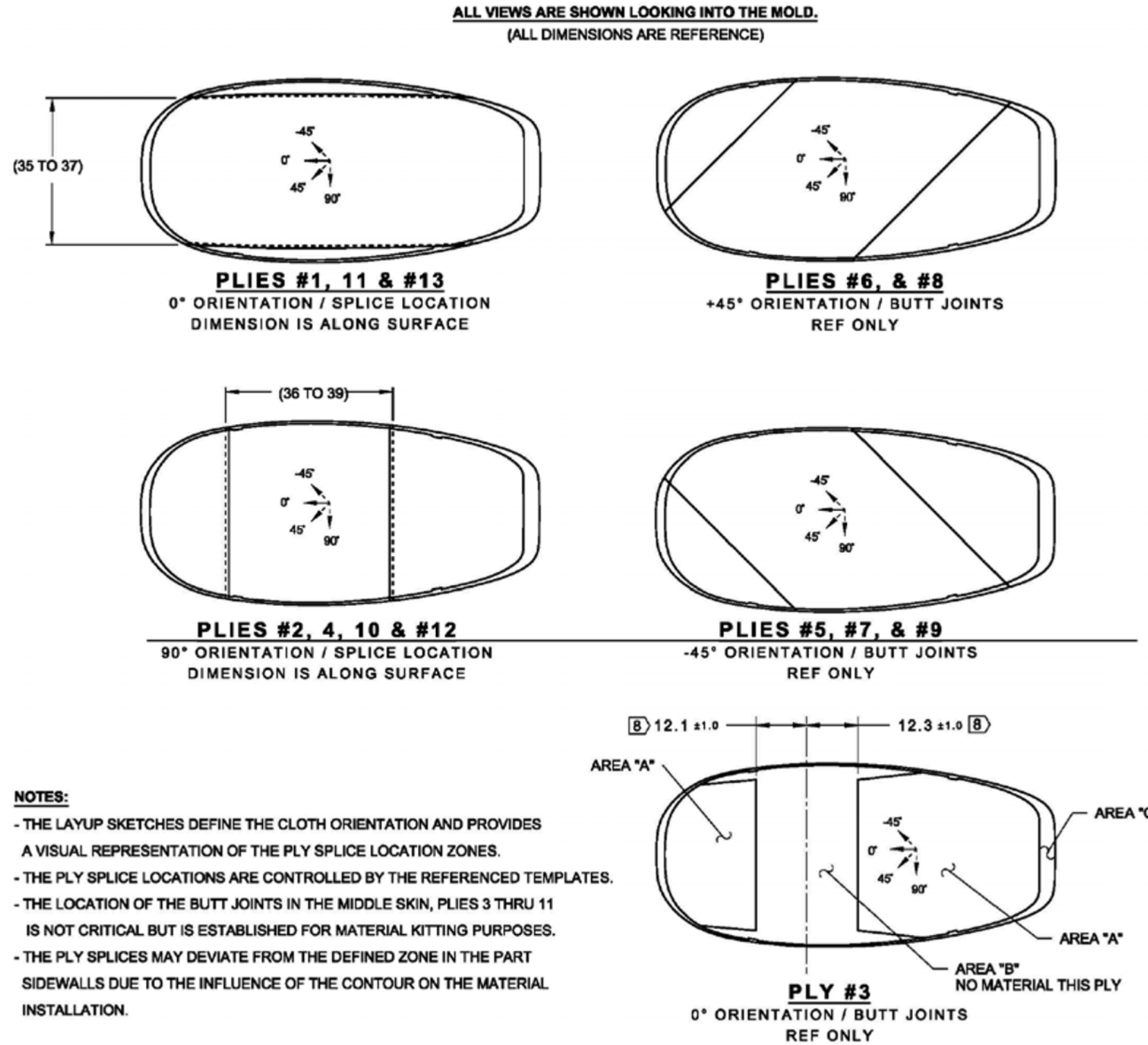
Figure 4-32. (Sheet 6 of 6) Fuselage Mount Radome Outline and Installation Drawing (90401395, REV D)
