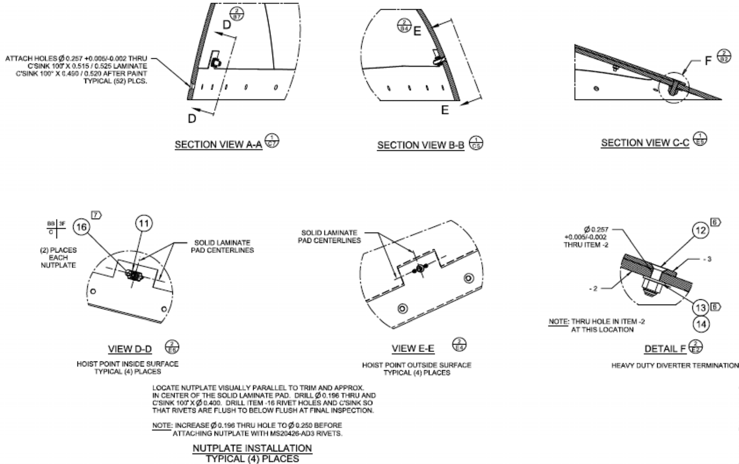
Figure 4-32. (Sheet 2 of 6) Fuselage Mount Radome Outline and Installation Drawing (90401395, REV D)
