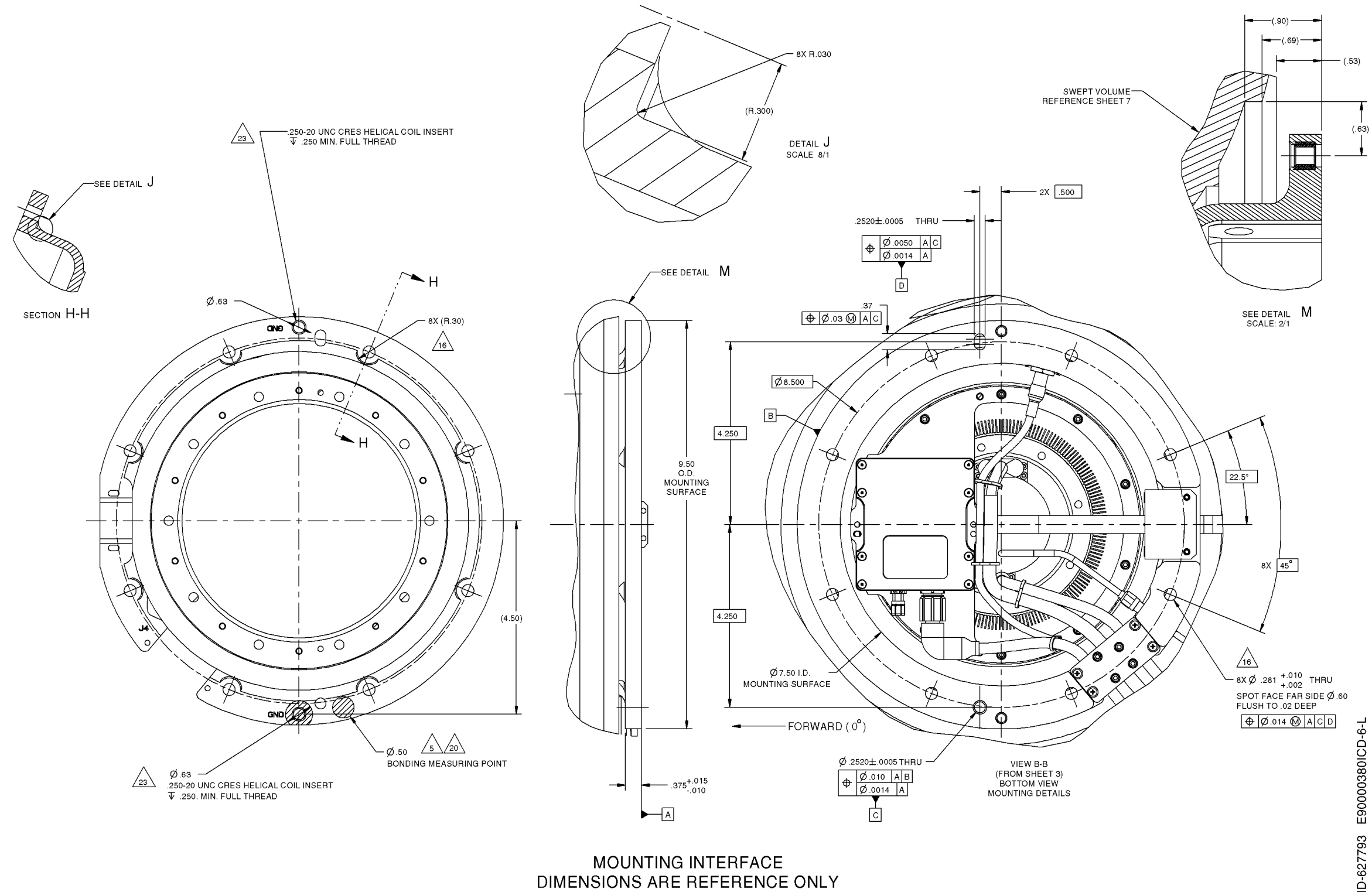
Figure 4-31. (Sheet 6 of 14) FMA Outline and Installation Drawing (90000380ICD, REV L)
