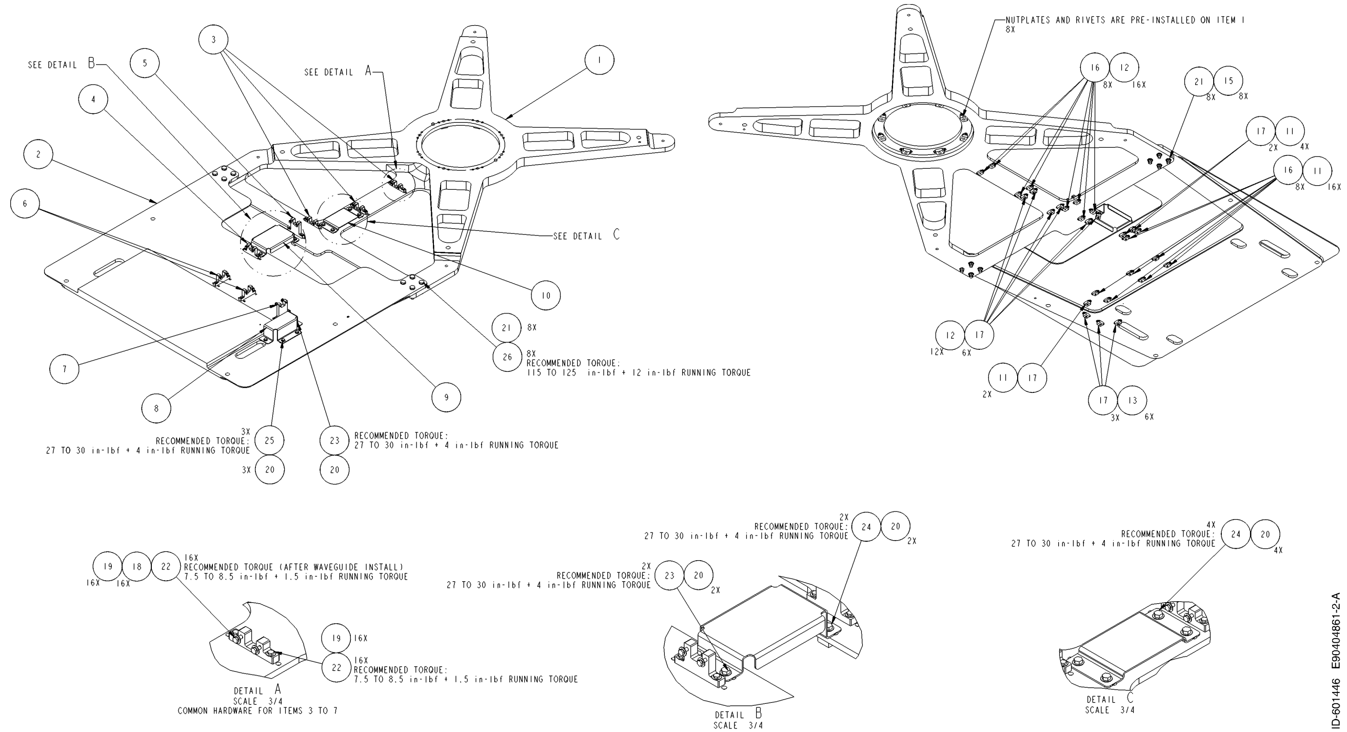
Figure 4-33. (Sheet 2 of 4) LAIM Outline and Installation Drawing (90404861, REV A)
