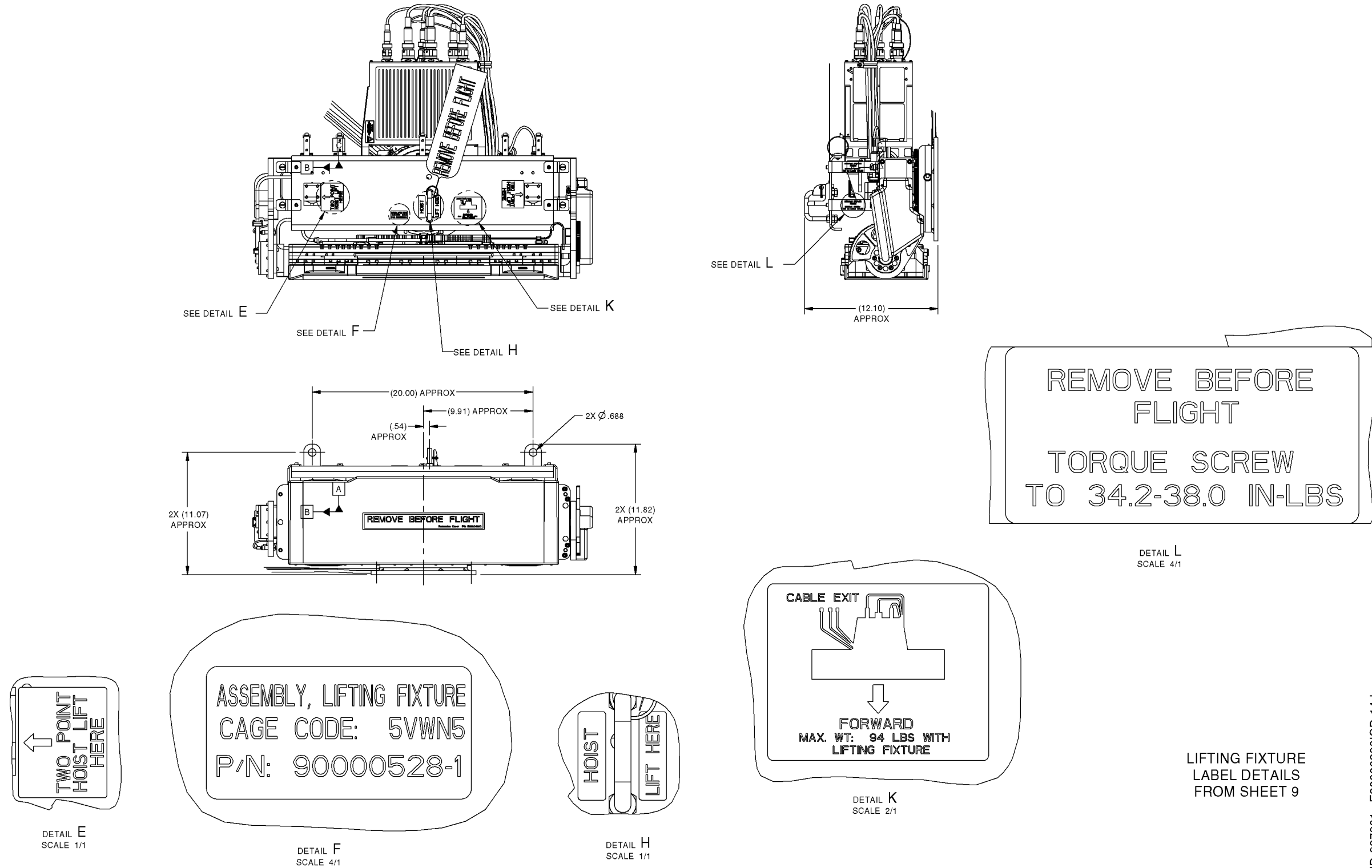
Figure 4-31. (Sheet 14 of 14) FMA Outline and Installation Drawing (90000380ICD, REV L)
