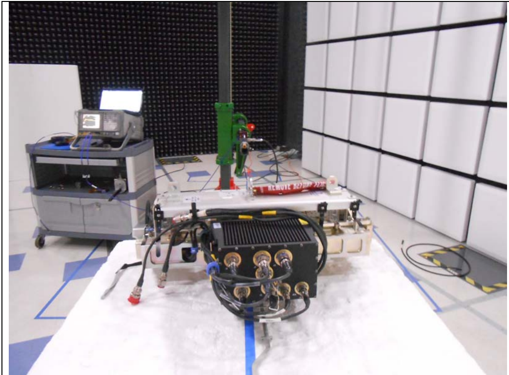
RF Radiated above 1 GHz with TMA Antenna #1
