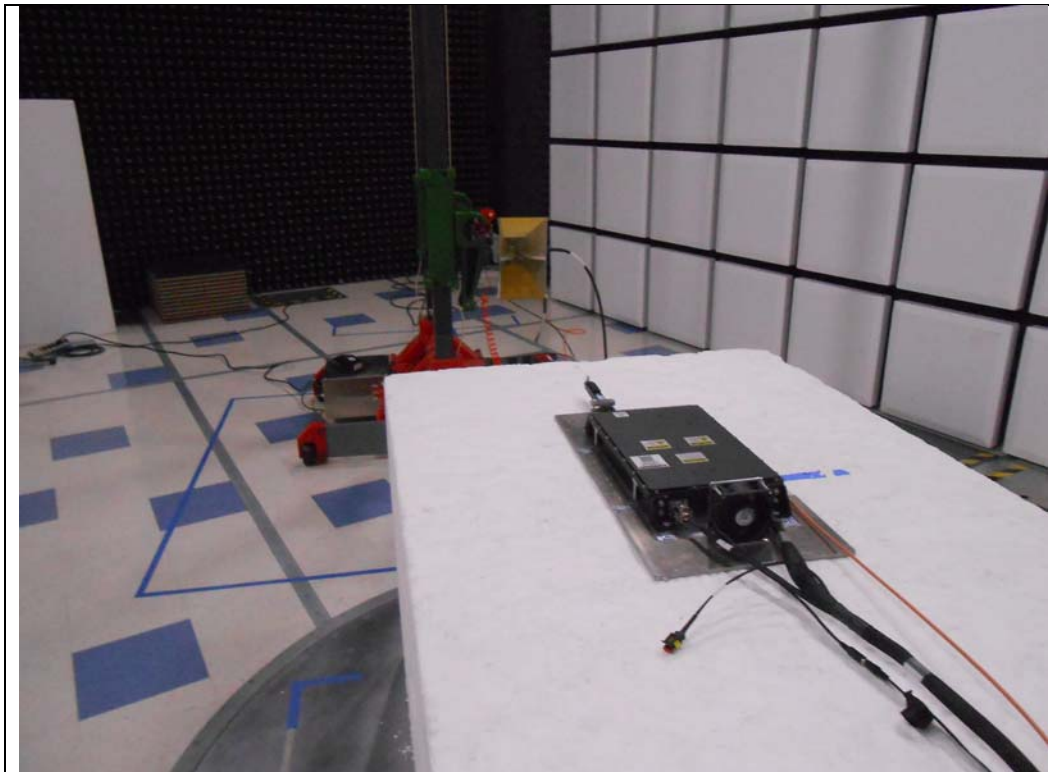
RF Radiated above 1 GHz with 50 ohm Load #1
