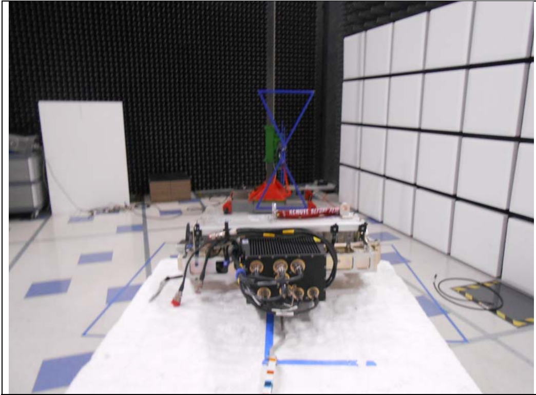
RF Radiated below 1 GHz with TMA Antenna
