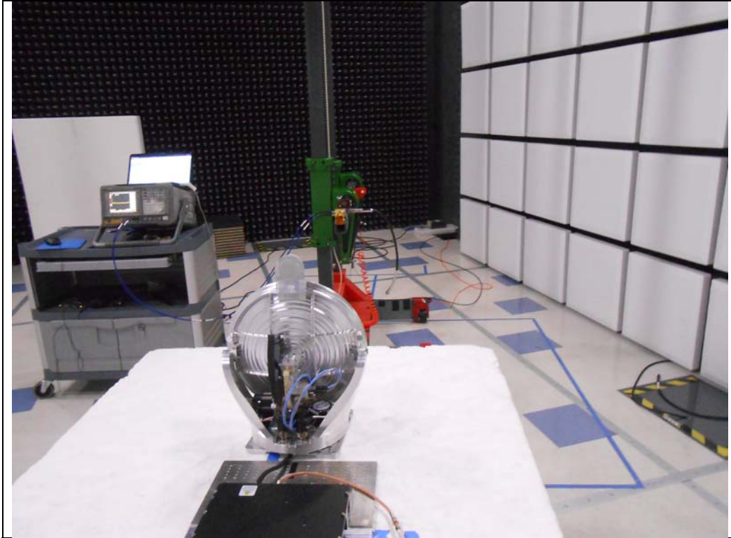
RF Radiated above 1 GHz with TMA Antenna #2
