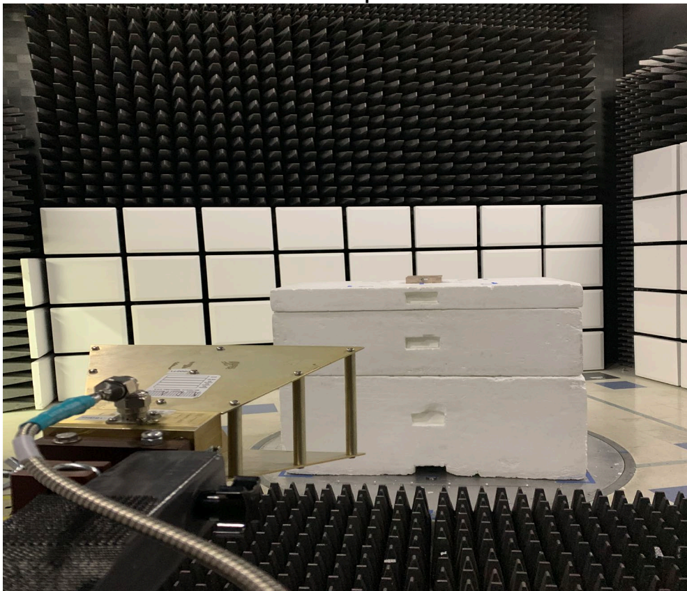
Radiated Setup 1-18Ghz
