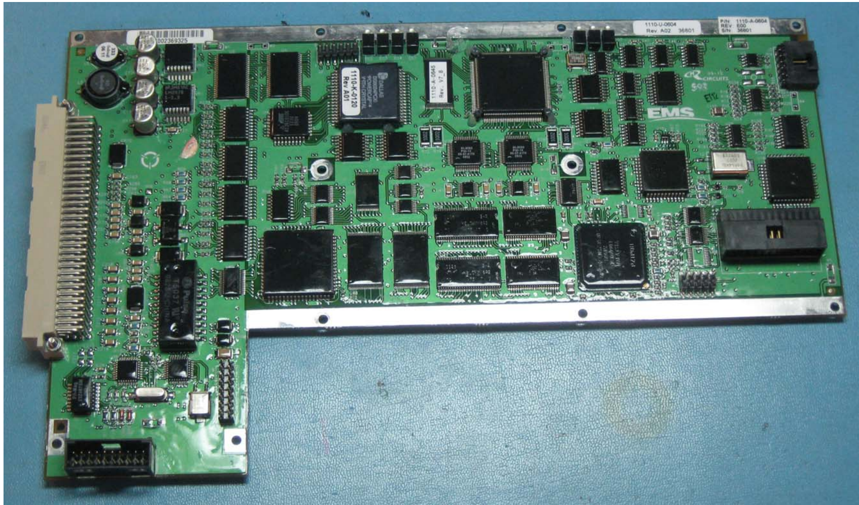
Figure 1: 1110-A-0604 Data Processor Top
