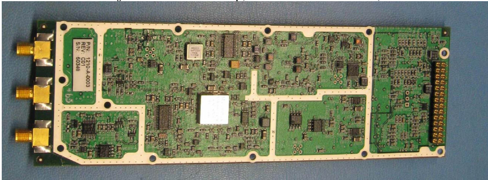
Figure 8: 1210-A-0003 RF Module Bottom (Part of the HST BGAN 1 Channel Card)
