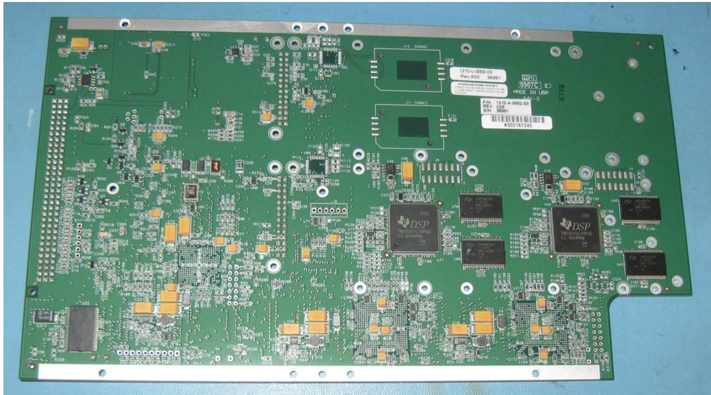
Figure 6: HST Digital Module 1210-A-0002-03 Bottom (Part of the HST BGAN 1 Channel Card)
