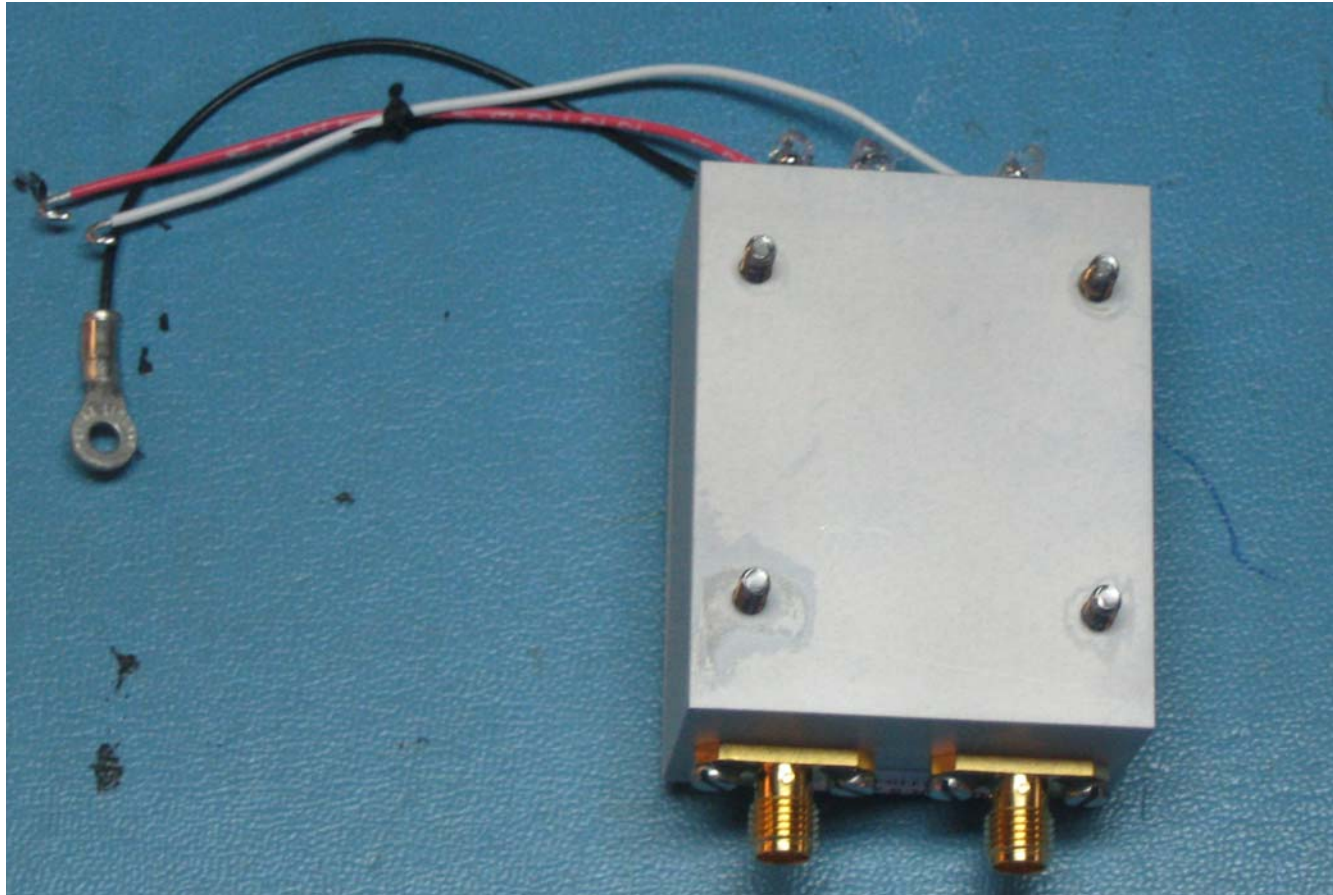
Figure 10: 1110-F-0617 OXCO Bottom
