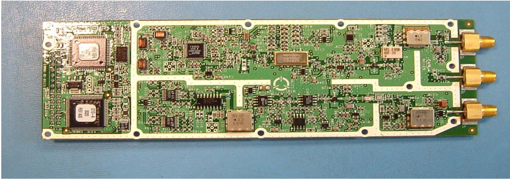
Figure 7: 1210-A-0003 RF Module Top (Part of the HST BGAN 1 Channel Card)
