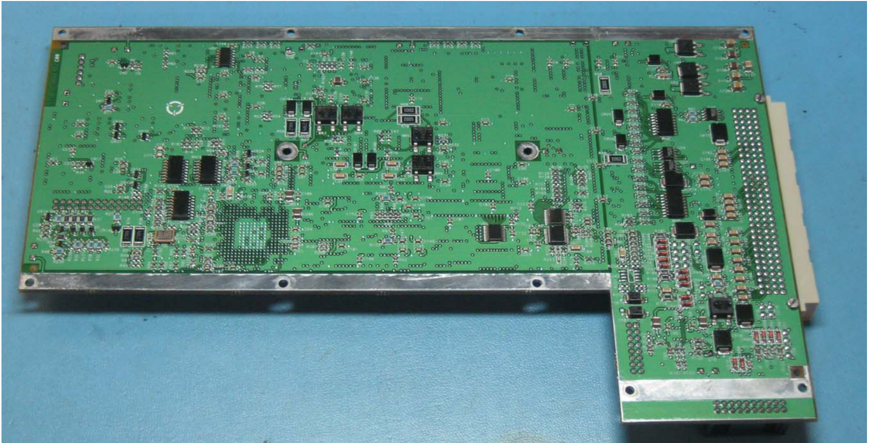
Figure 2: 1110-A-0604 Data Processor Bottom
