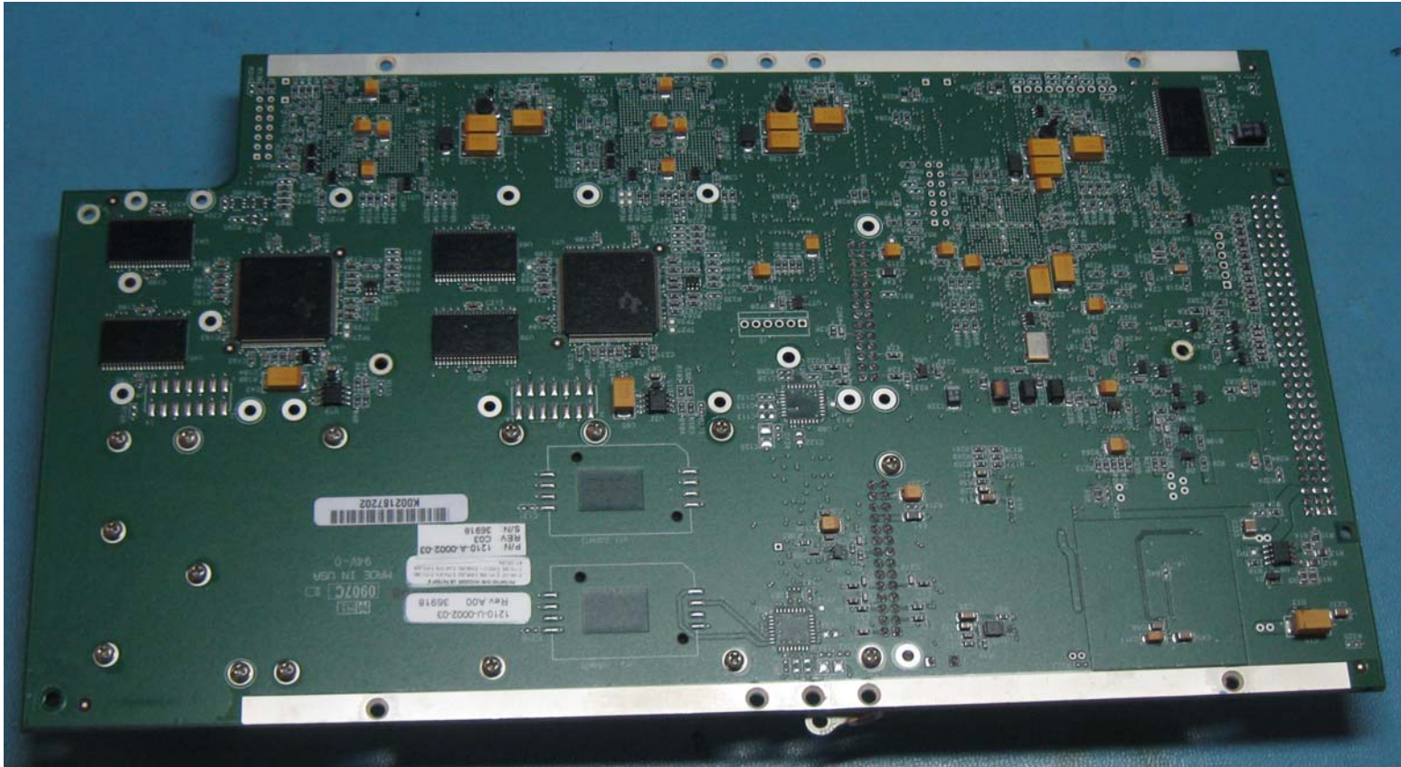
Figure 4: 1210-A-0010-03 HST BGAN 1 Channel Card Bottom
