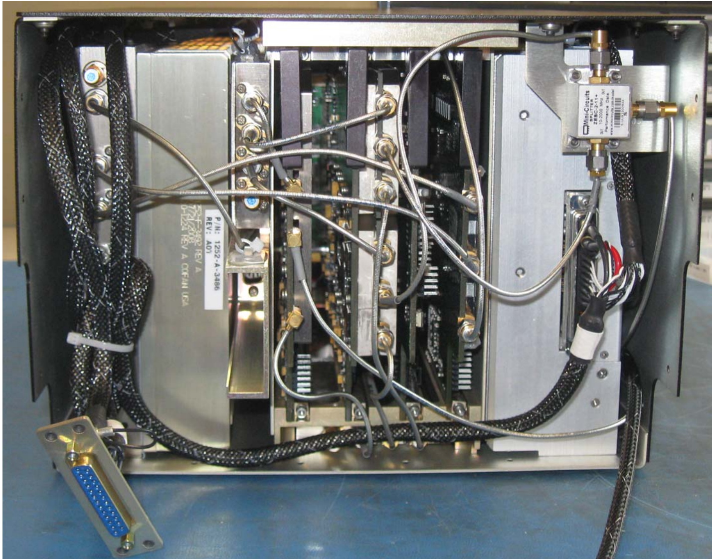
Figure 23: Interconnections
