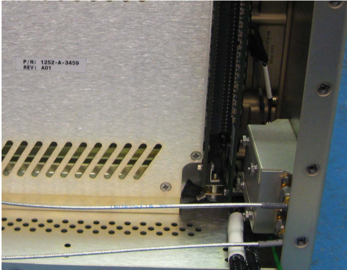
Figure 17: OXCO Installed
