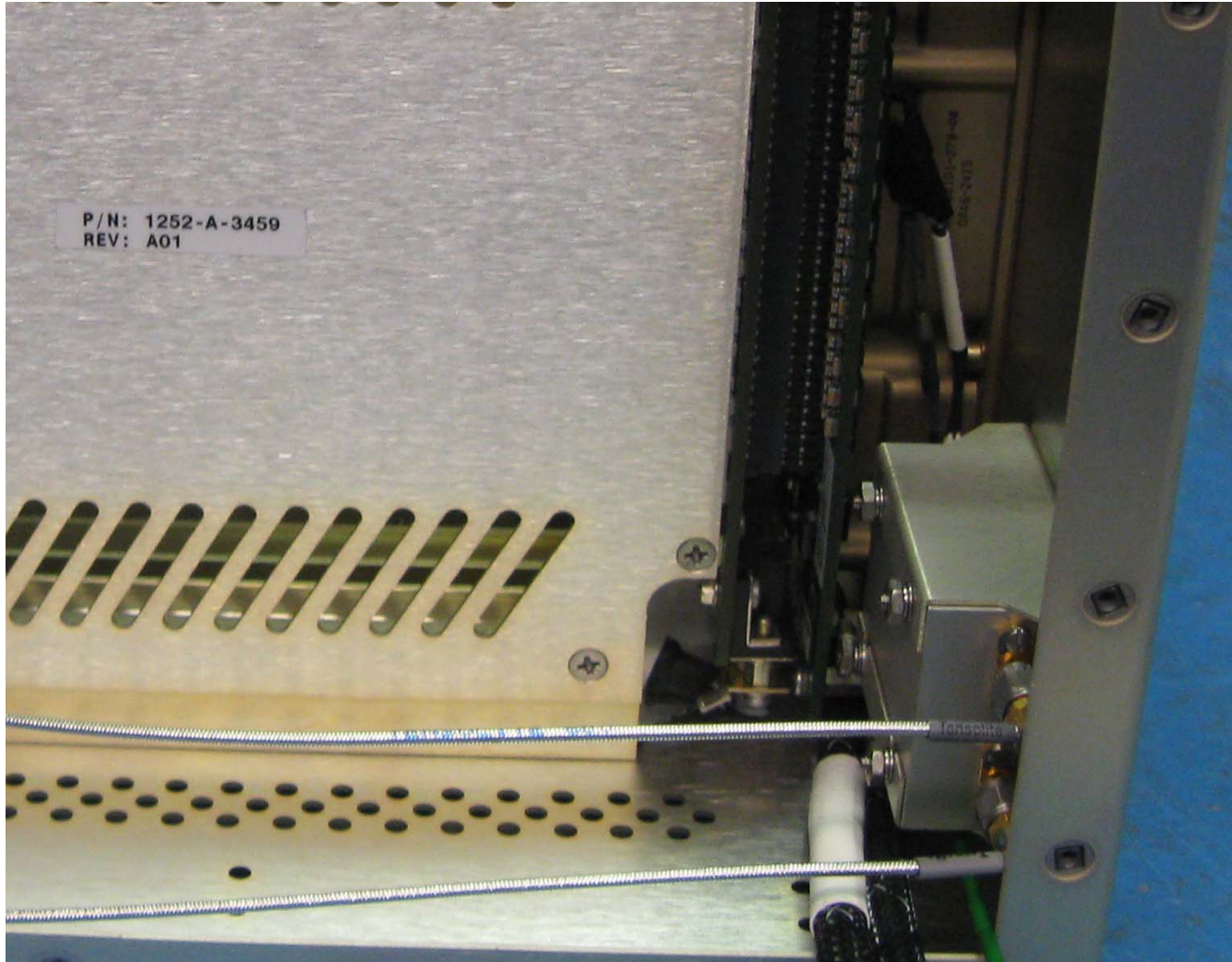
Figure 17: OXCO Installed
