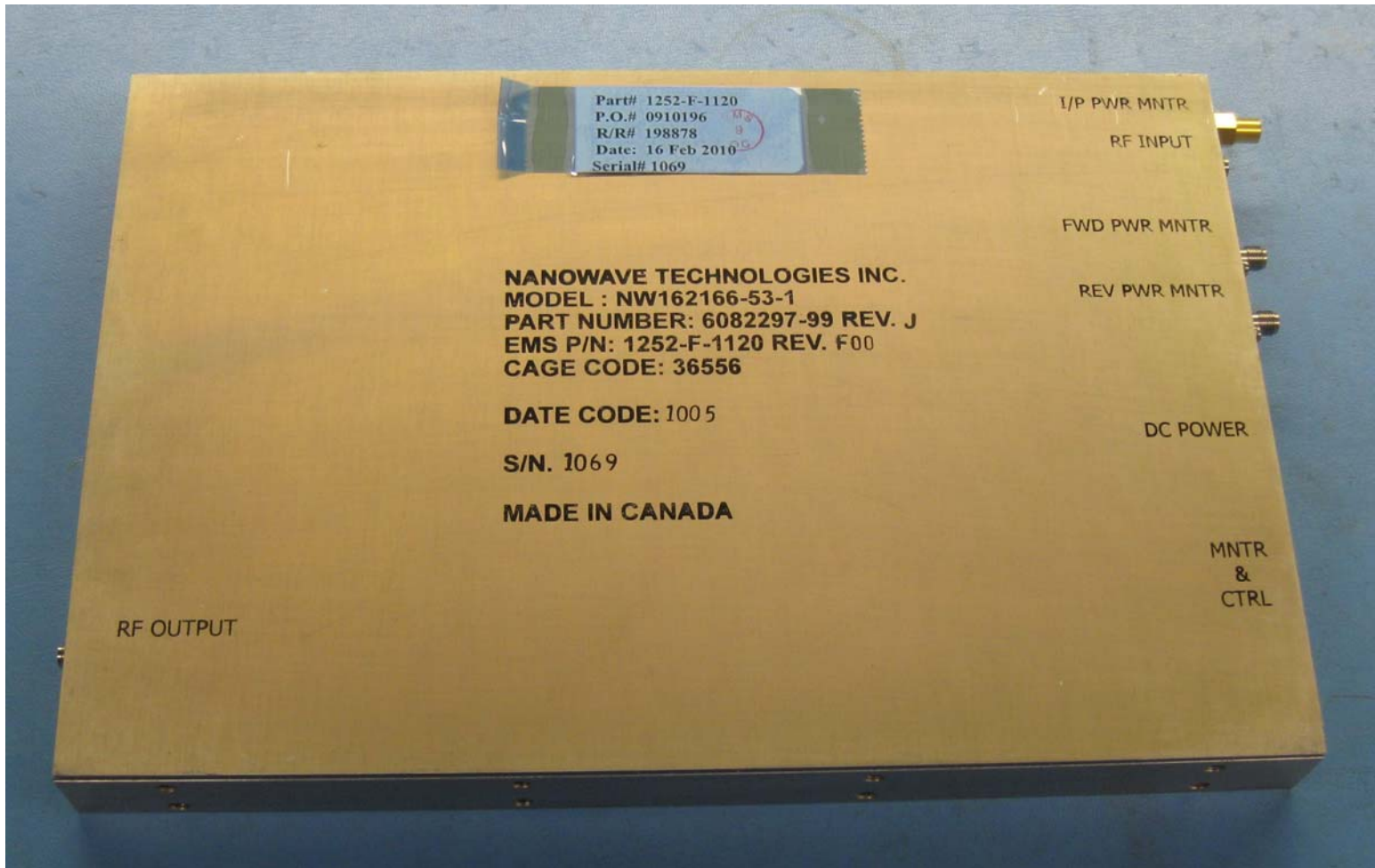
Figure 20: Power Amplifier Top
