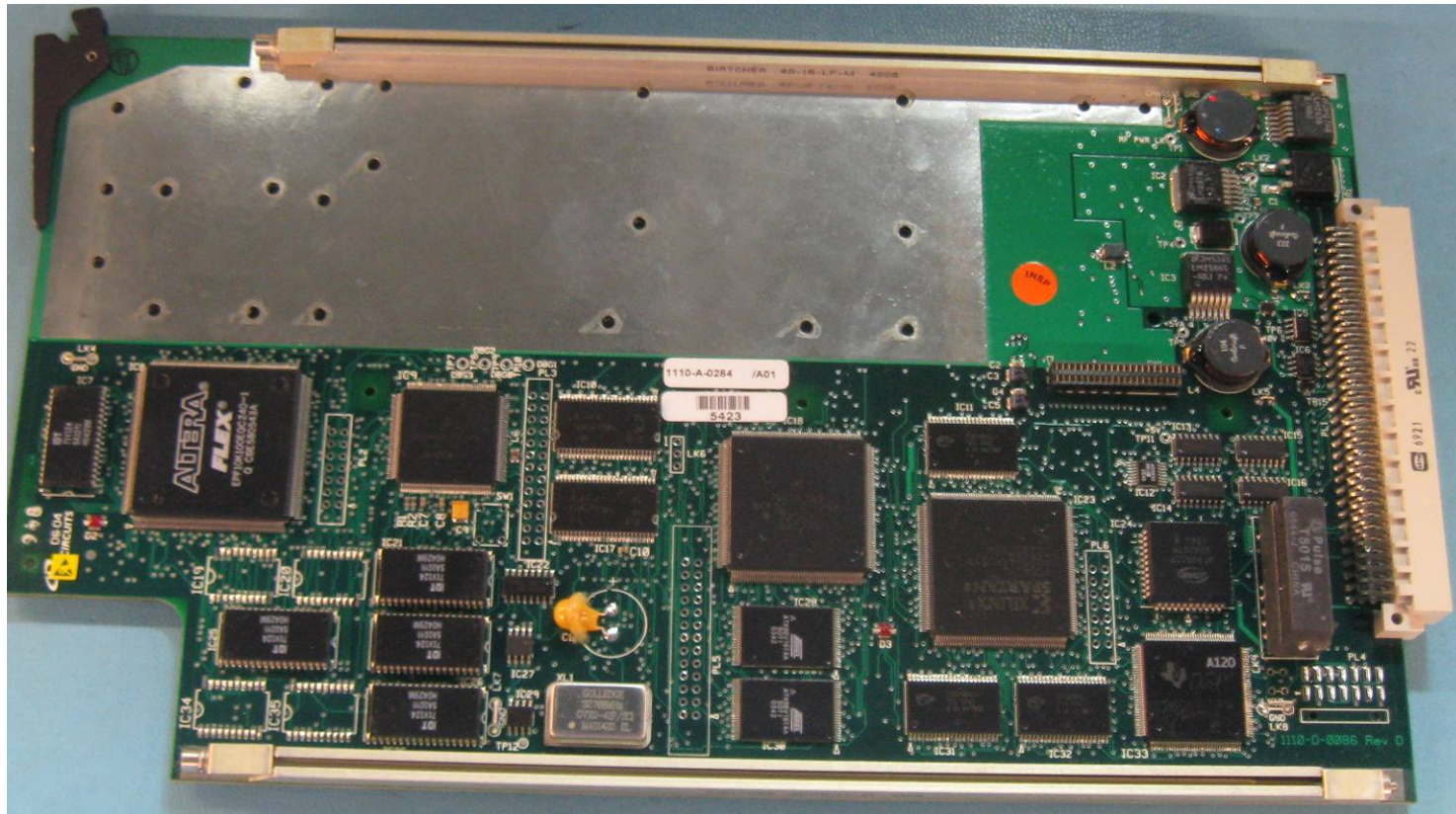
Figure 5:1110-A-0284 HSD Digital Module Top (Part of the AERO Channel Card)
