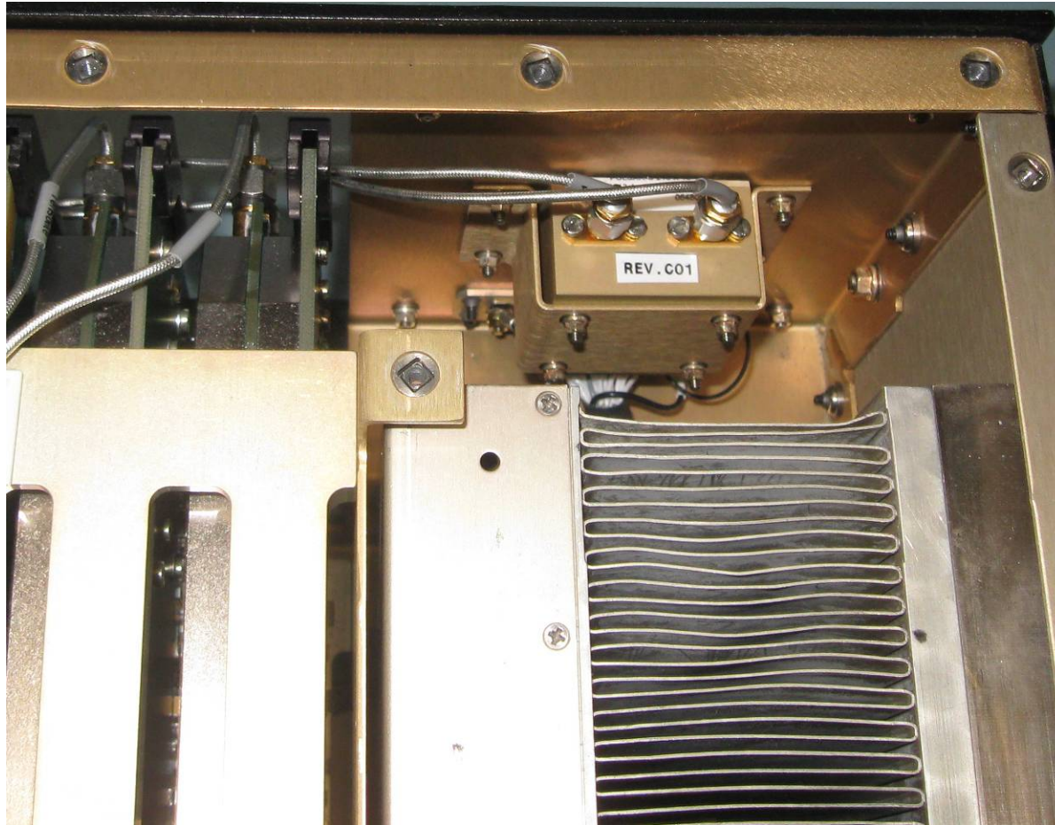
Figure 11: 1110-F-0017 OXCO Installed
