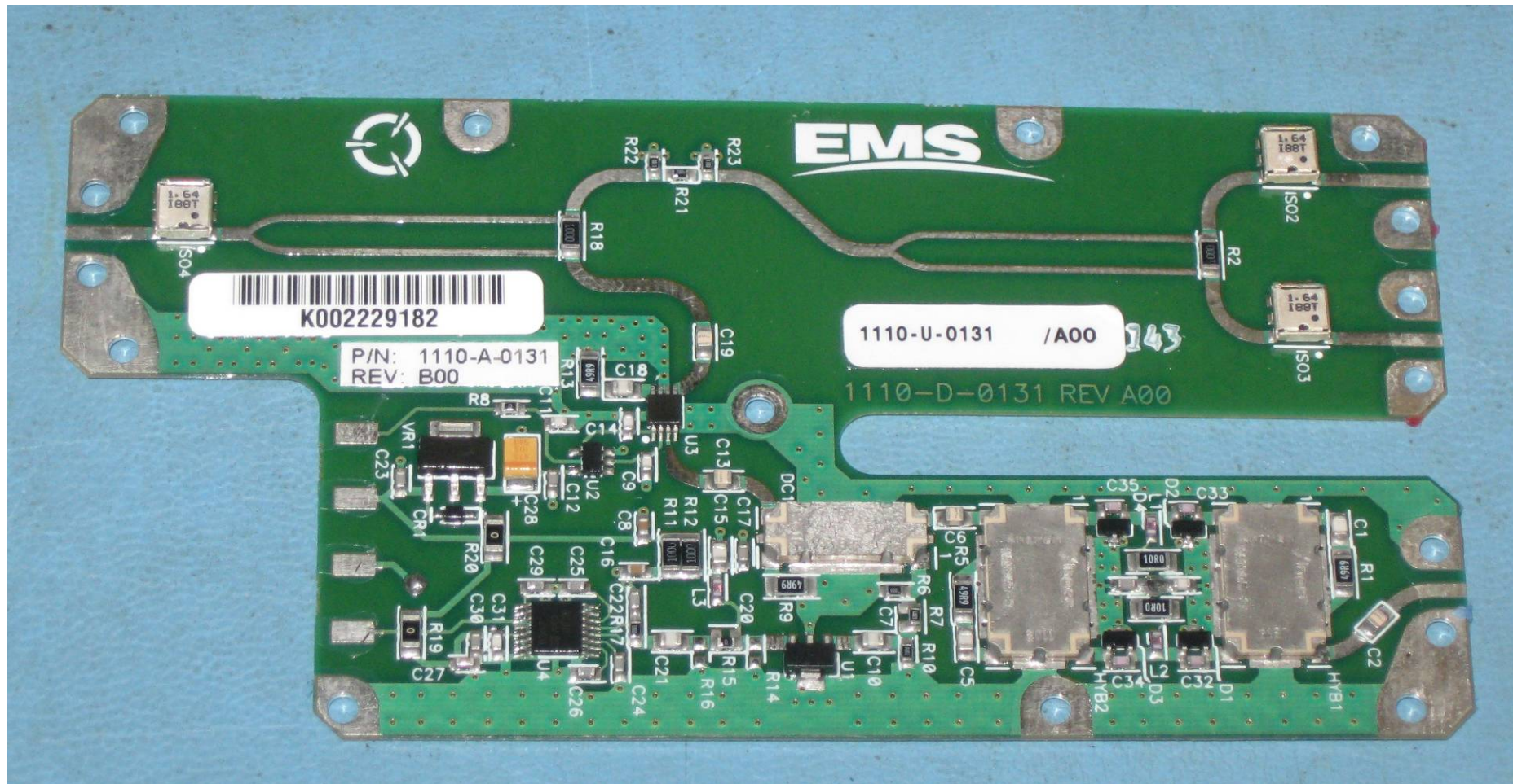
Figure 17: 1110-A-0130 _1110-A-0131 CCA RF Card (Part of the RF Control Module)
