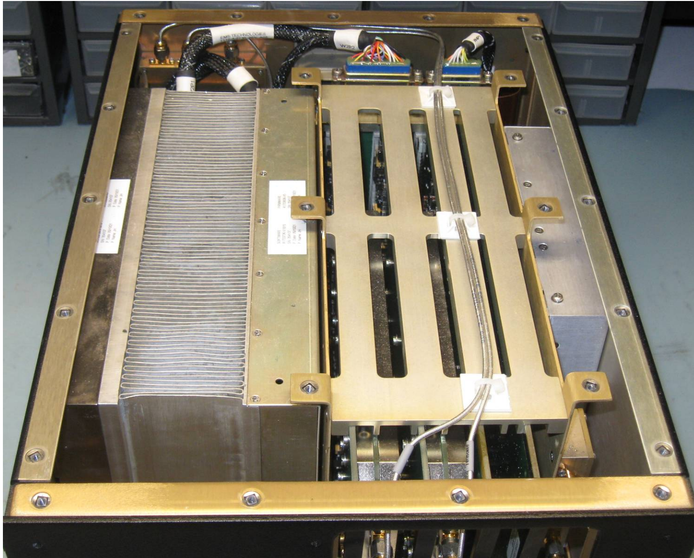
Figure 22: Interconnections Top View
