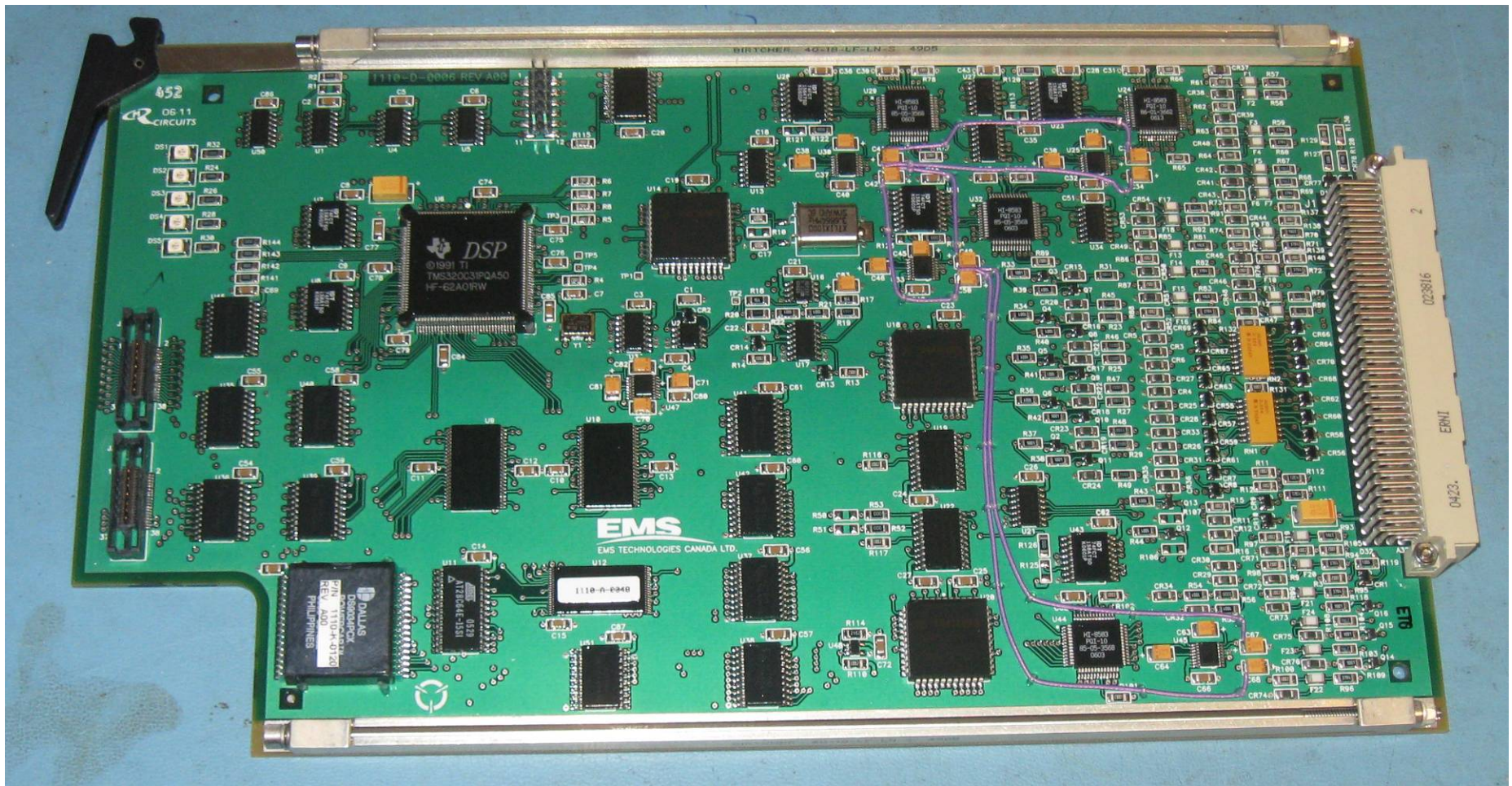
Figure 1: 1110-A-0006 Control Processor Top
