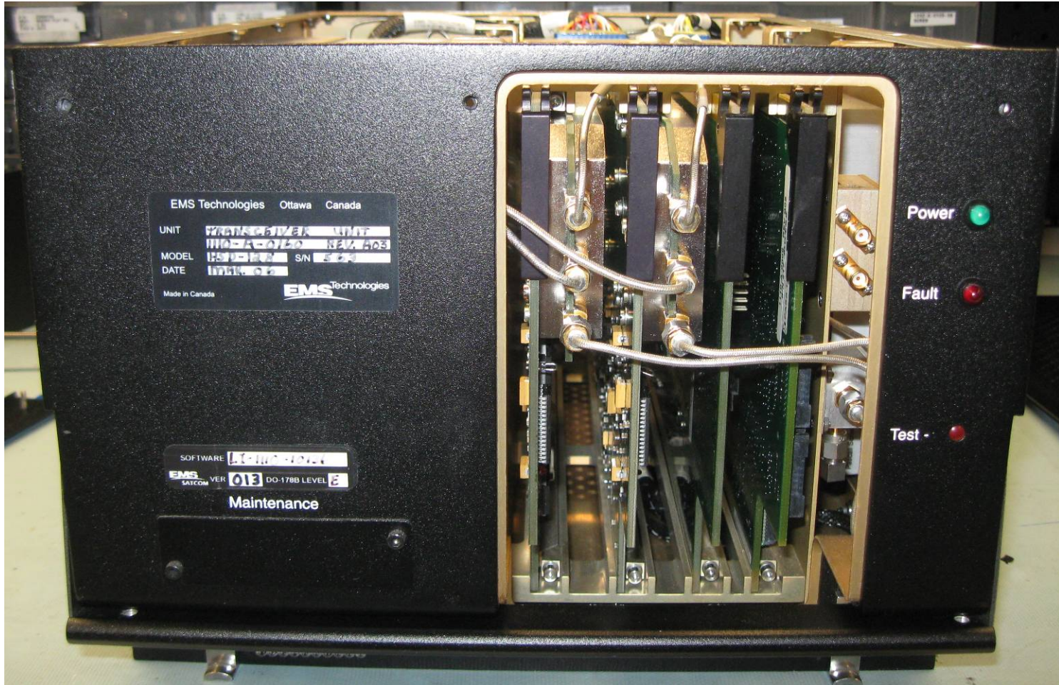
Figure 21: Interconnections Front View
