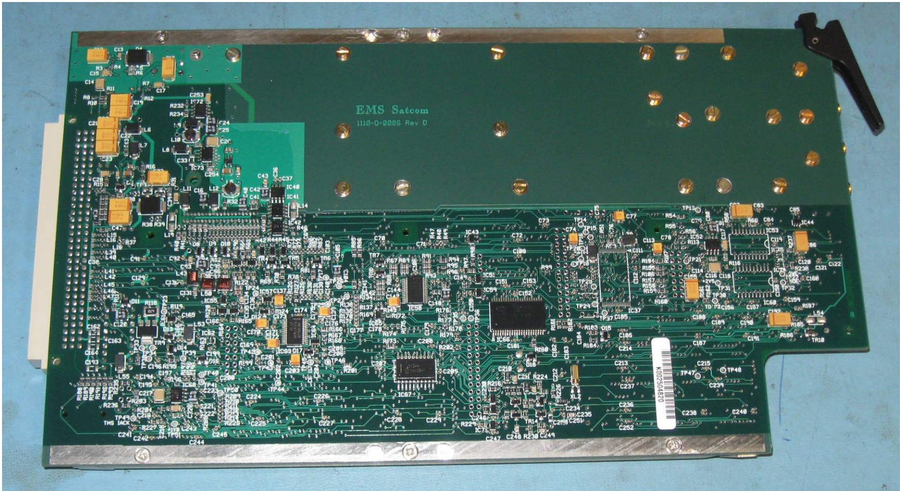
Figure 4: 1110-A-0004 Channel Card Bottom
