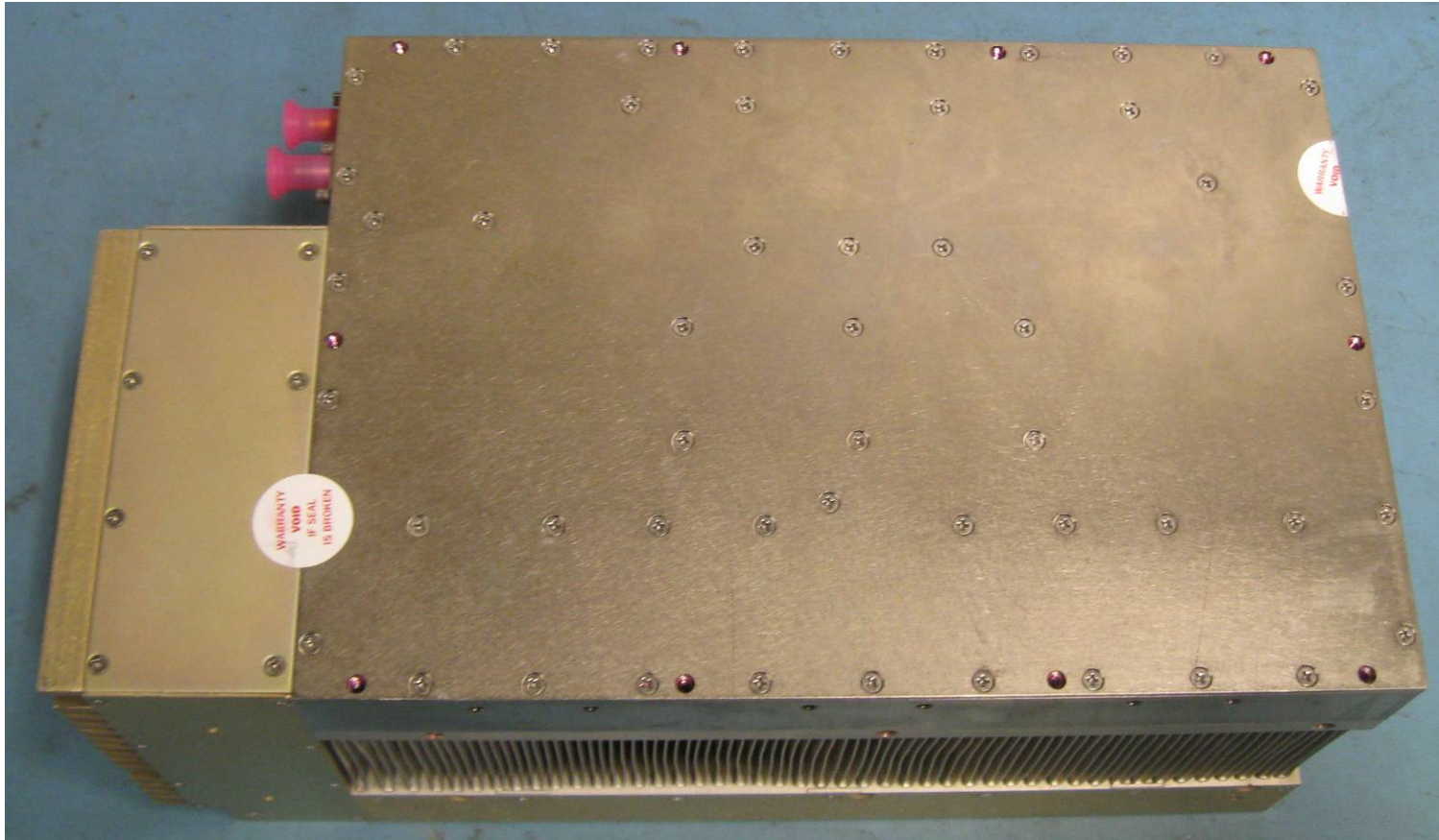
Figure 15: 1110-F-0073 HPA Bottom
