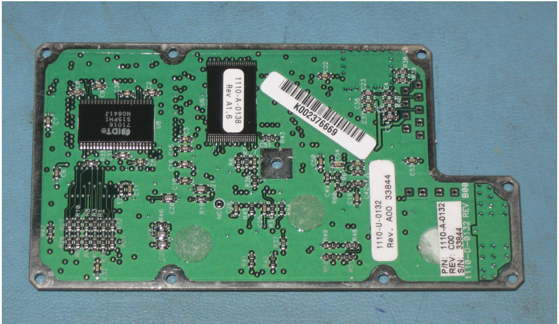
Figure 19: 1110-A-0130 _1110-A-0132 Control Card CCA Bottom (Part of the RF Control Module)
