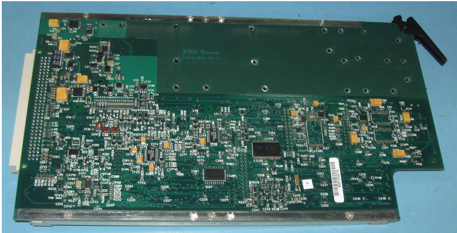
Figure 6: 1110-A-0284 HSD Digital Module Bottom (Part of the AERO Channel Card)
