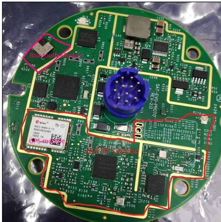
Photo 4: EUT displaying the all the RF sections
