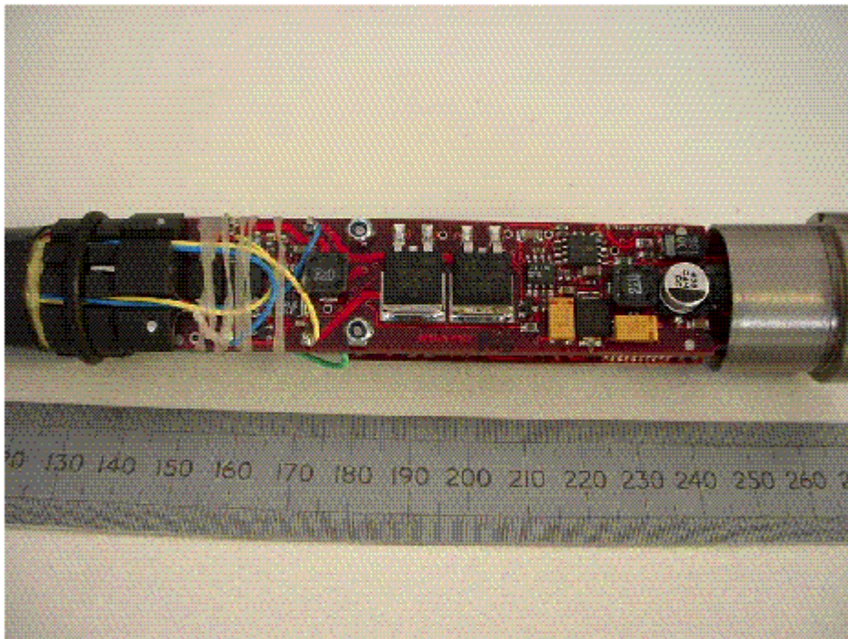
Photograph 2 TX PCB Track Side
