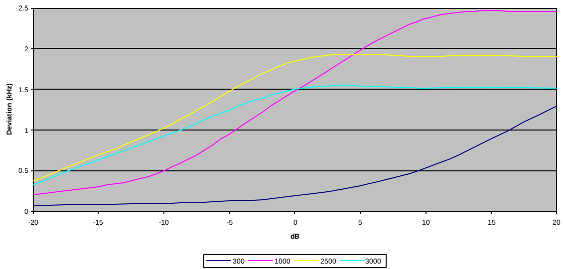
Modulation Limiting (429.975 MHz; 12.5 kHz channel spacing; Negative Peak)
