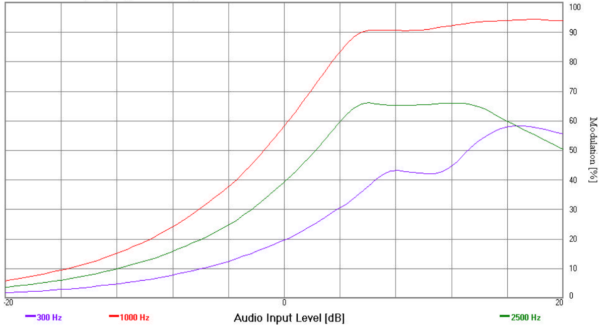
RTL AM Modulation Limiting Response [121.5 MHz.] - Negative Peak
