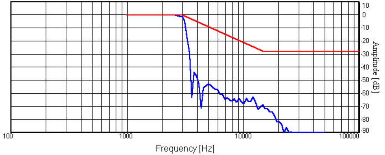
RTL Audio Low Pass Filter Response (160.1 MHz ; 12.5 kHz Channel Spacing)
