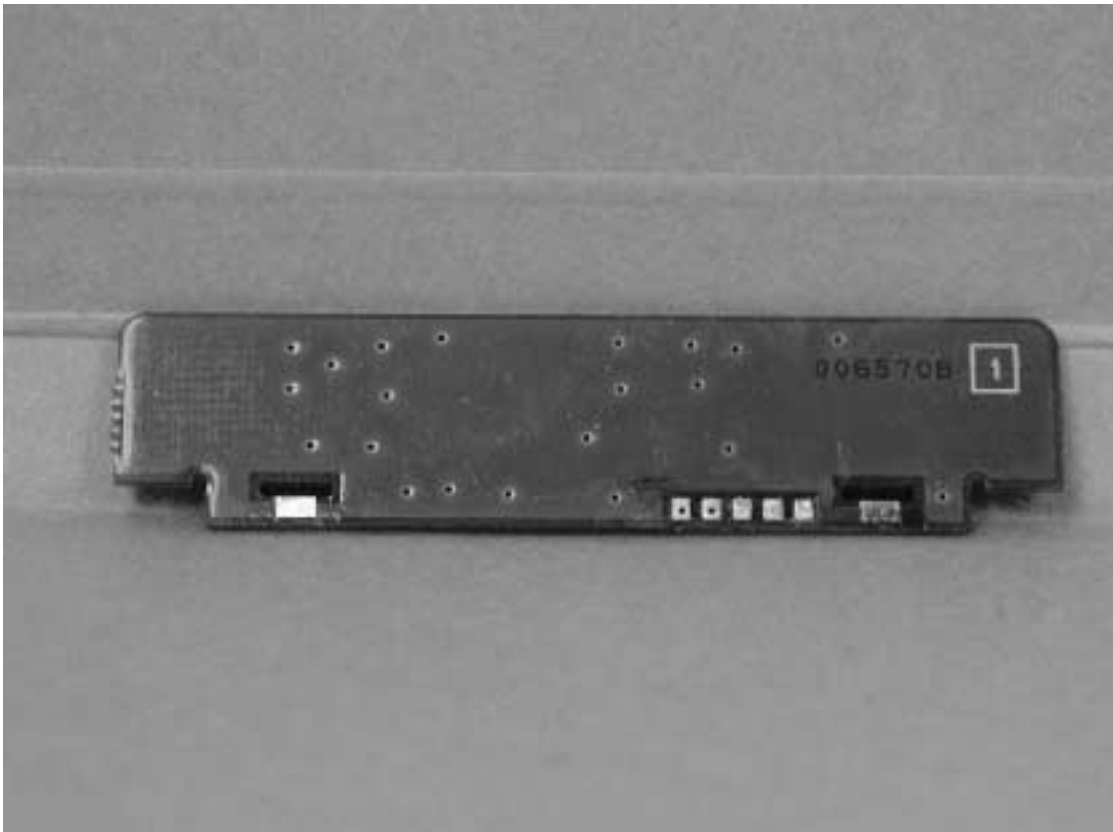
Solder Side of SW-UNIT
