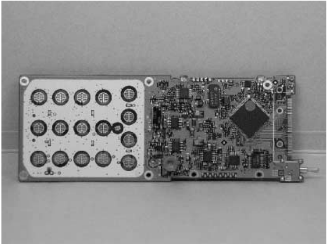
Top of PCB Board without LCD/VR/SW/Shield Case
