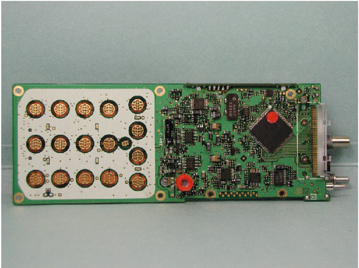
Top of PCB Board
