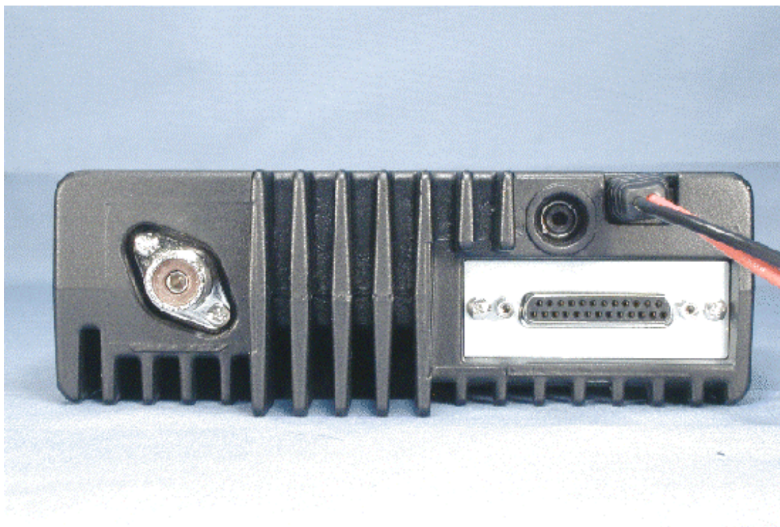
Rear view
