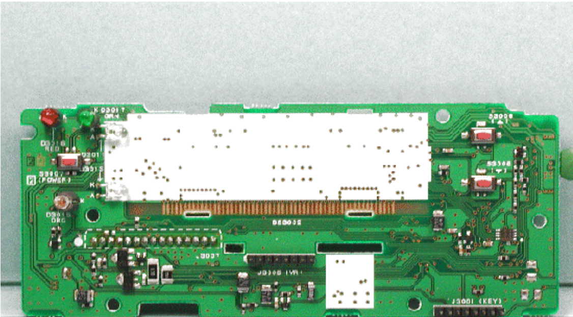
Side-A of DISPLAY-UNIT without LCD
