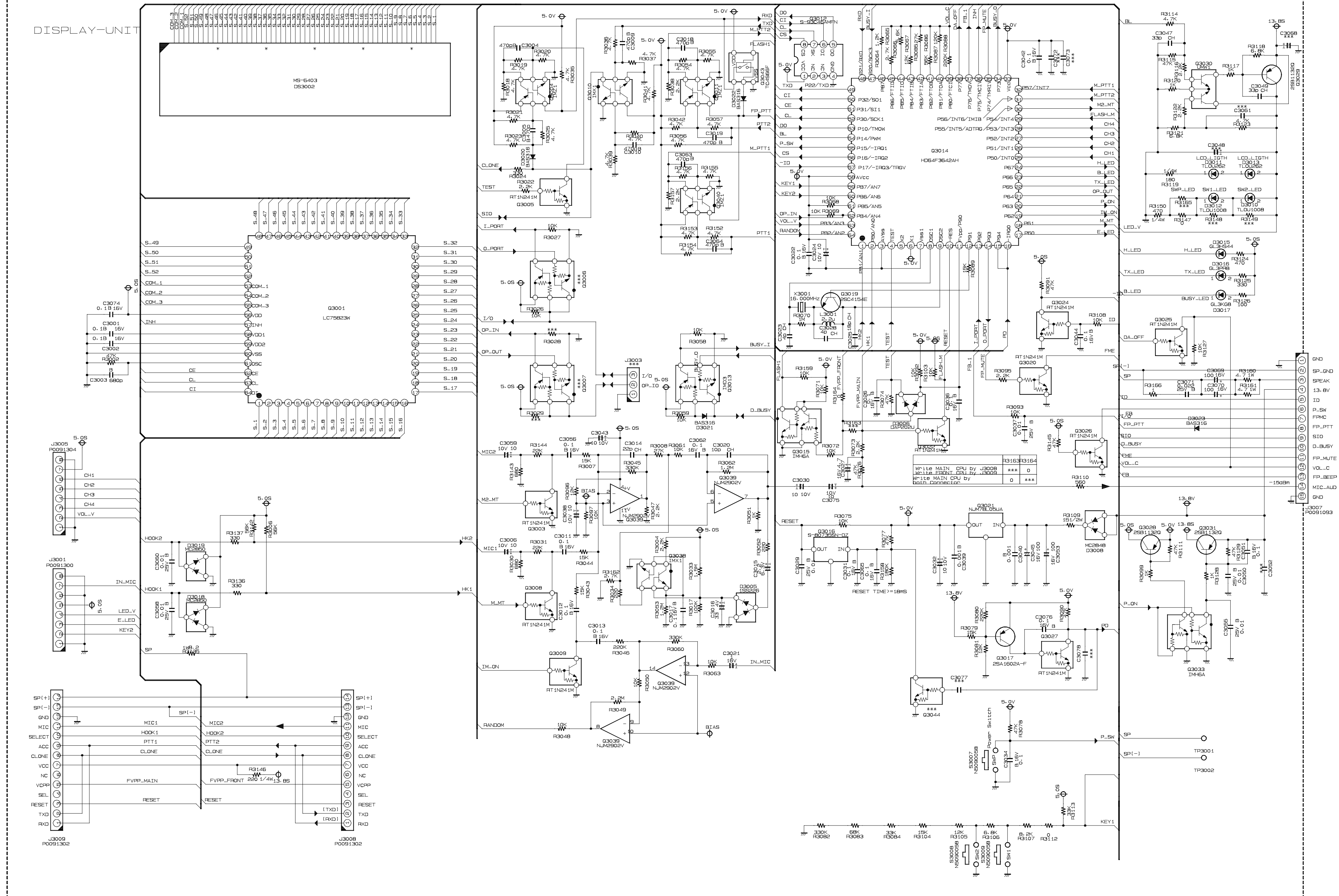
CIRCUIT DIAGRAM MODEL VX-4000 DES. B-AC005L000/DISPLAY-UNIT REF. BP006130E.cir/001.sht EDITION DATE 11 DEC. 2000 UPDATE 11 DEC. 2000 VERTEX STANDARD CO., LTD.
