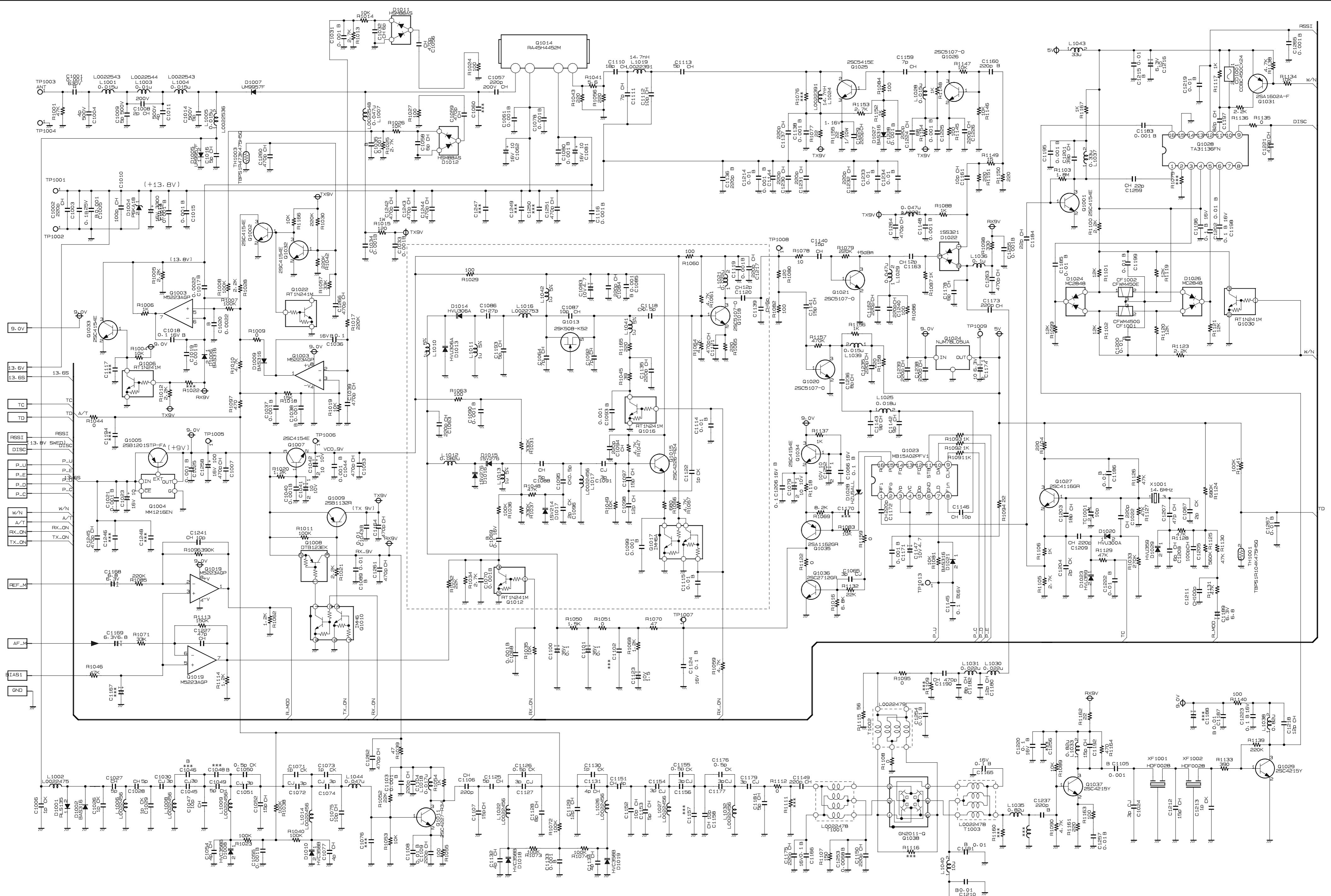
CIRCUIT DIAGRAM MODEL VX-3200U DES. B-AC039U000/RF-UNIT REF. BR008060B.cir/001.sht EDITION DATE 28 AUG. 2001 UPDATE 27 NOV. 2001 VERTEX STANDARD CO., LTD.
