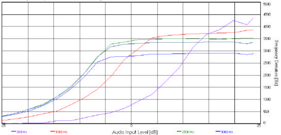
Modulation Limiting Response (467.525 MHz; 25 kHz Channel Spacing) Positive Peak
