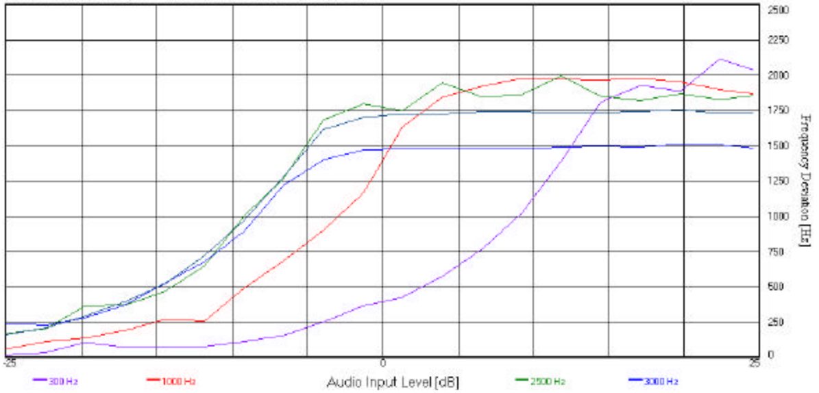
Modulation Limiting Response (467.525 MHz; 12.5 kHz Channel Spacing) Negative Peak
