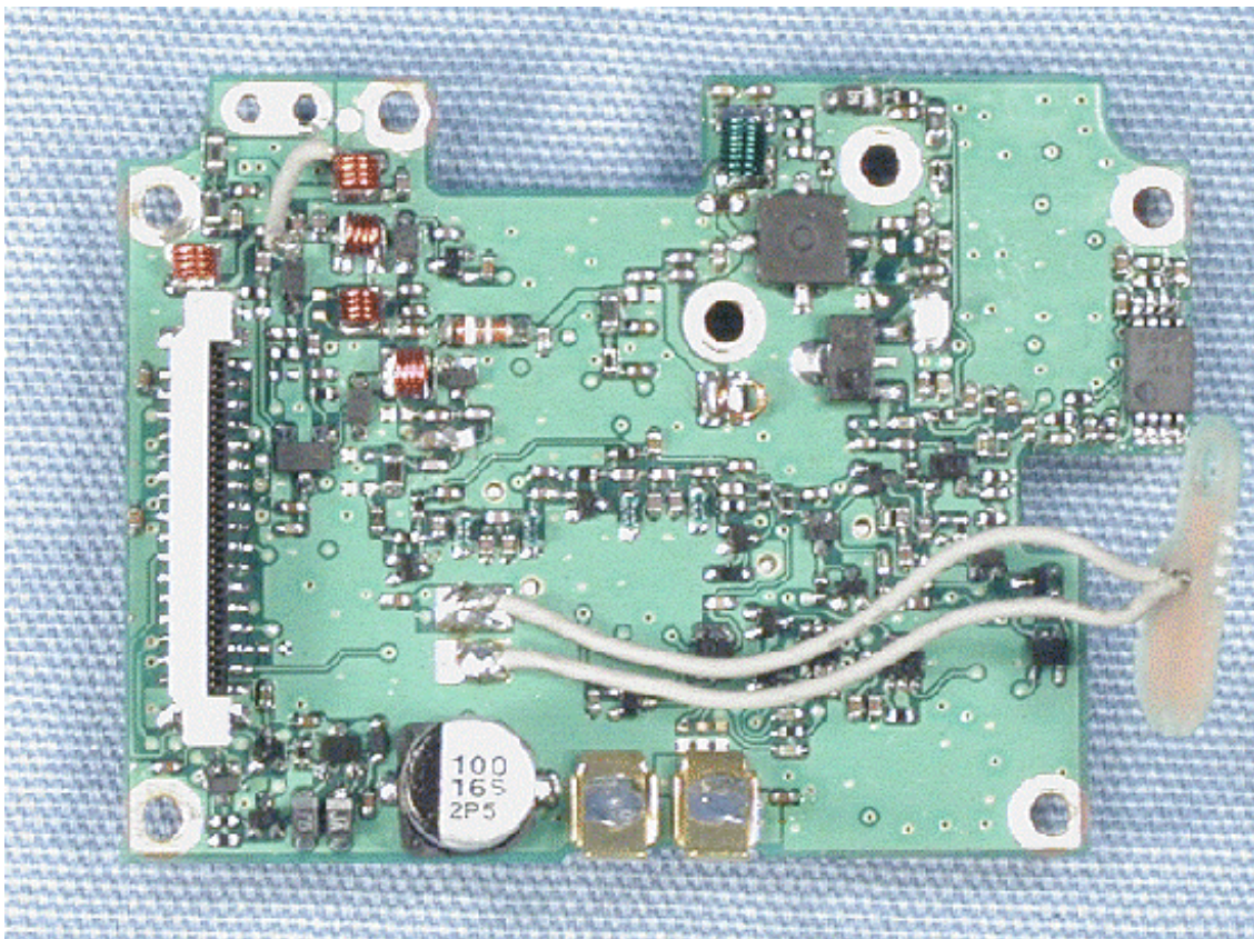
Side-A of RF-UNIT with SW-UNIT
