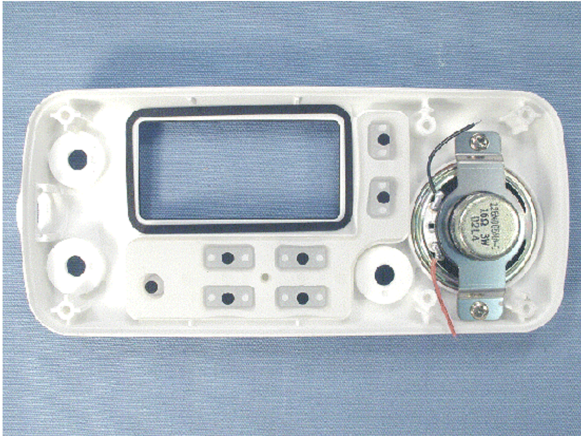
Inside of Panel without PWB
