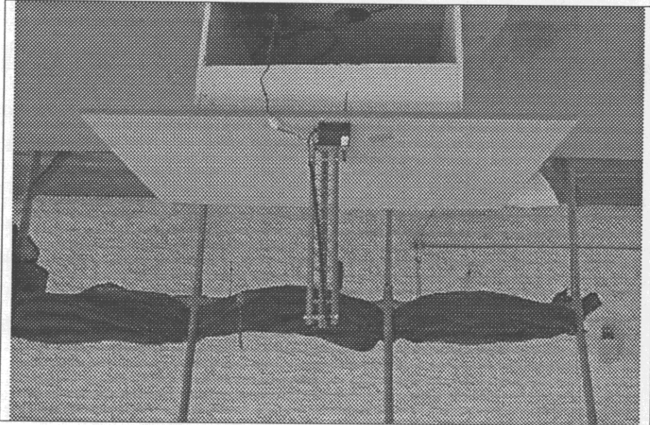
TEST SETUP: Radiated Emissions g9920030: 1999-Feb-05 Fri 03:13:12 STATE: 0:General
