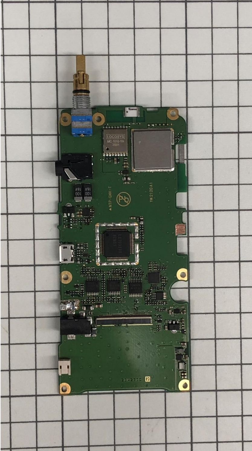
CNTL-UNIT
