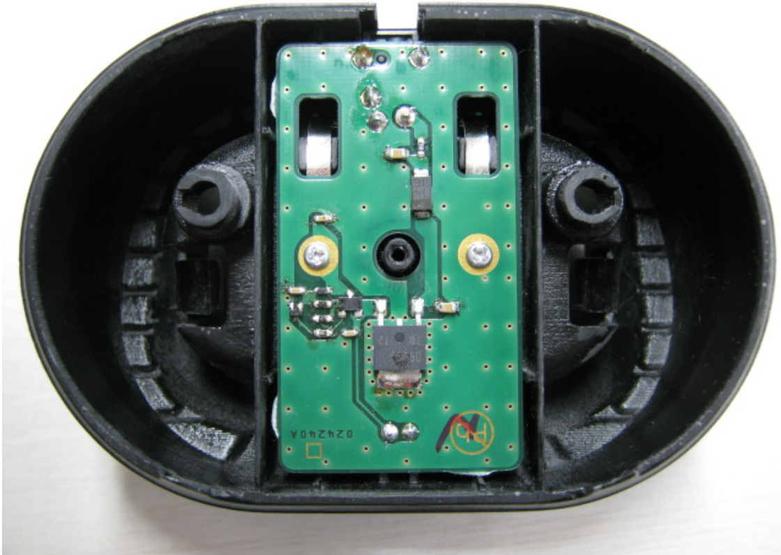
Inside of Charger (CD-57)
