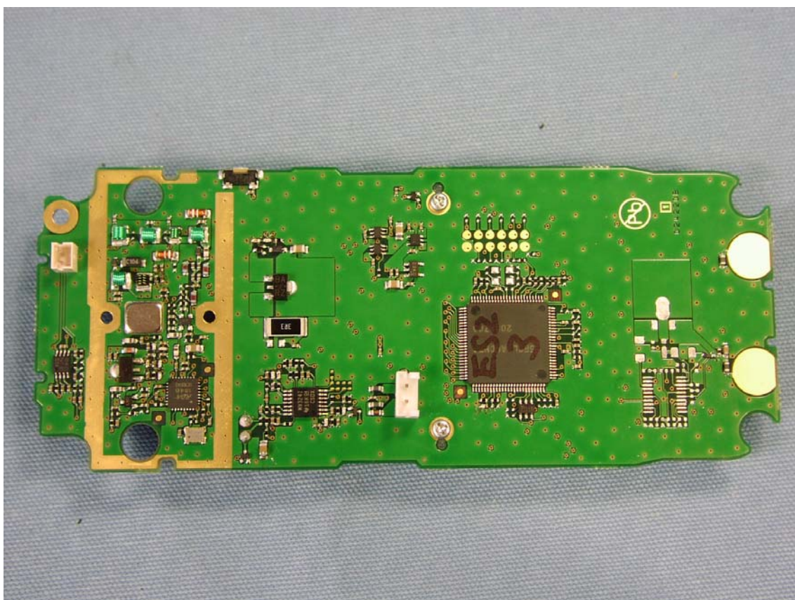
Side-B of MAIN-UNIT without chassis
