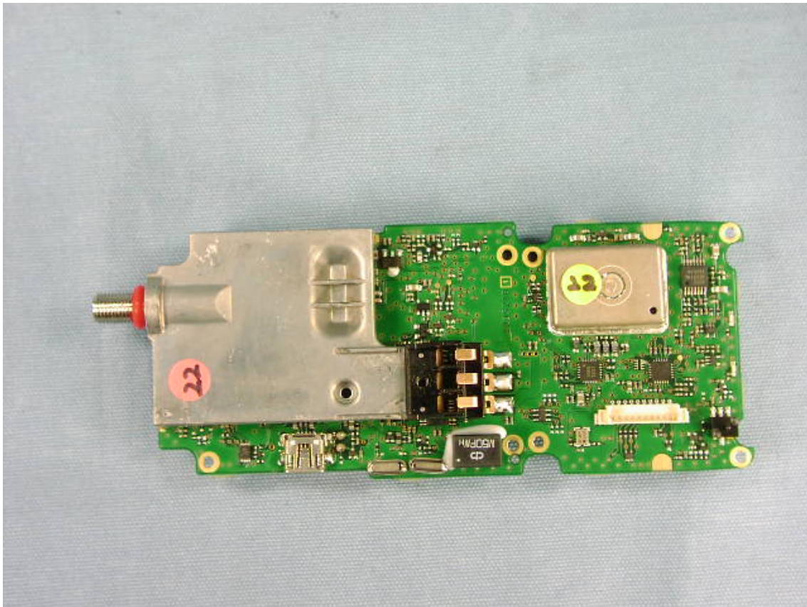
Side-B of MAIN-UNIT with chassis and Shield Cover
