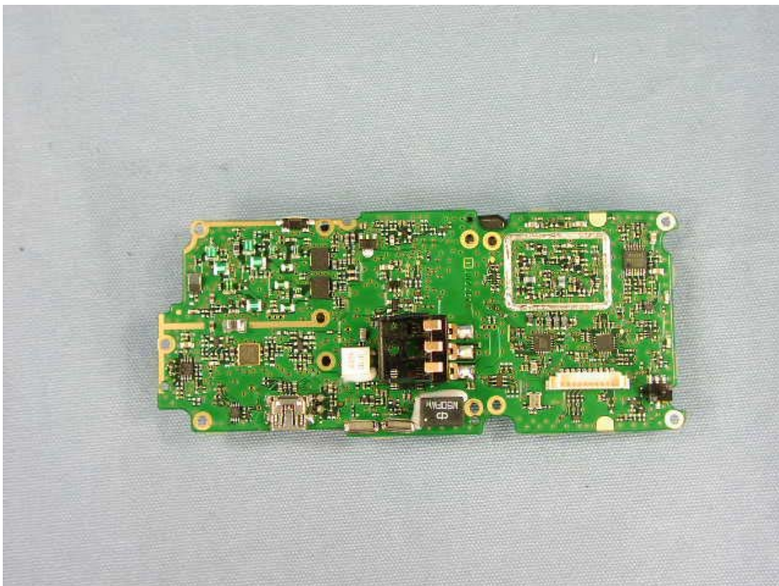
Side-B of MAIN-UNIT without chassis and Shield Cover
