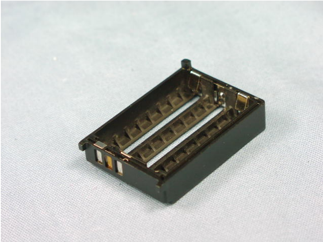
Alkaline Battery Case (FBA-44)
