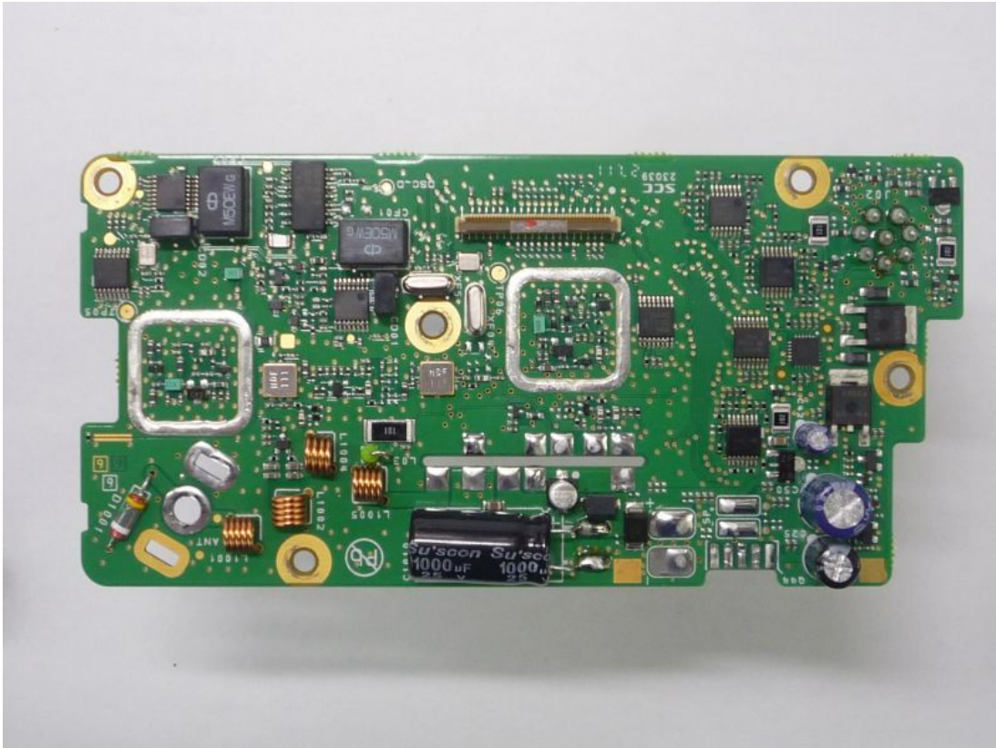
Side-A of MAIN-UNIT without shield cases
