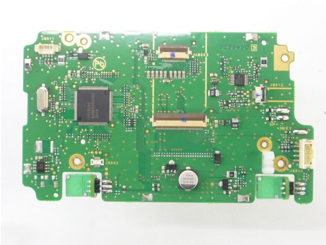
Side-B of CNTL-2-UNIT (GX1700 old GPS-UNIT Ver.)
