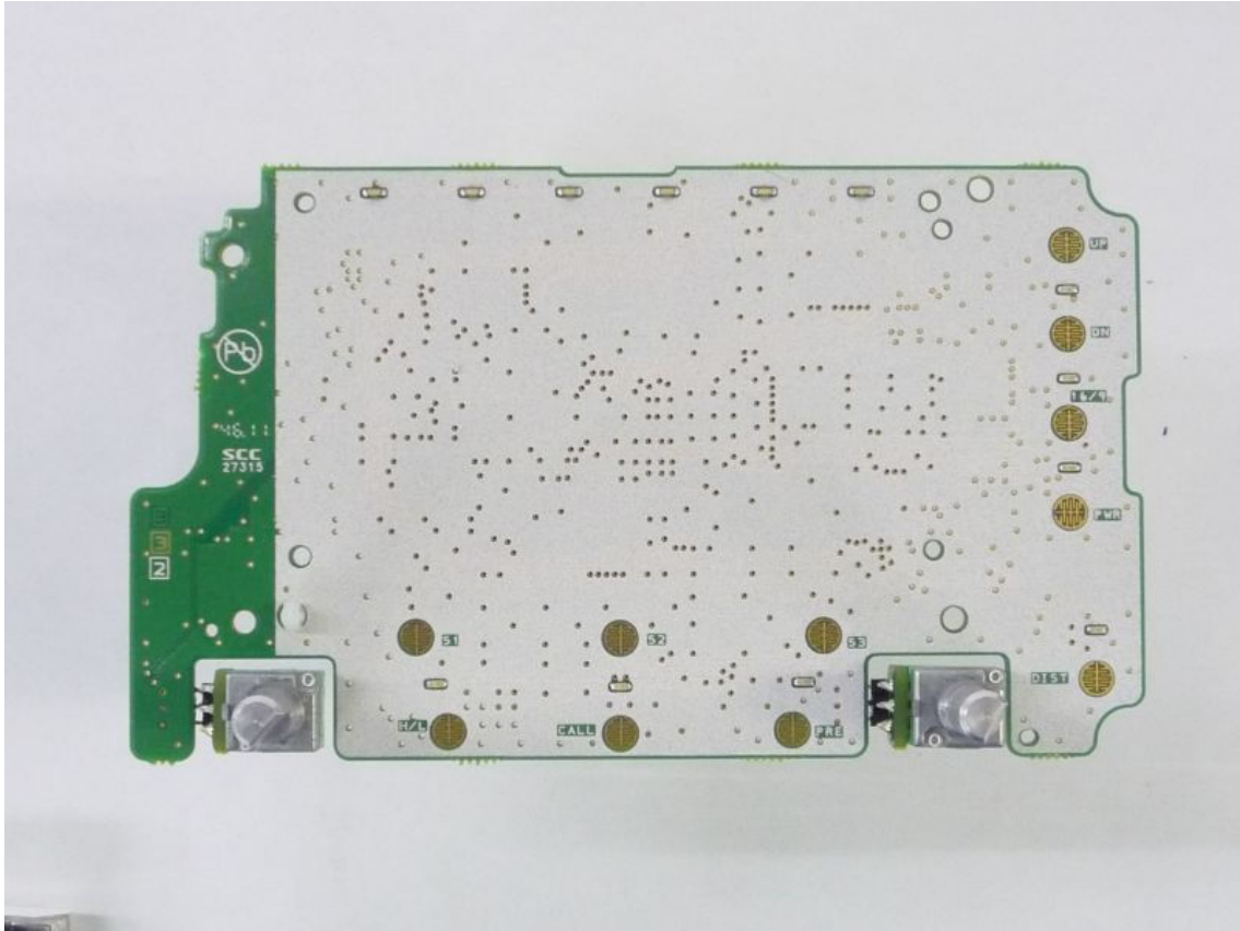
Side-A of CNTL-2 UNIT without LCD (GX1700 new GPS-UNIT Ver.)
