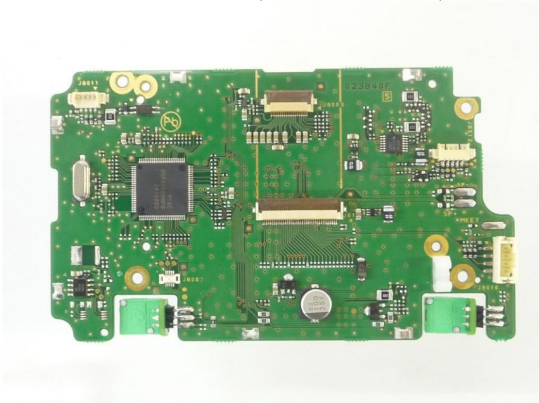
Side-B of CNTL-2-UNIT (GX1700 new GPS-UNIT Ver.)
