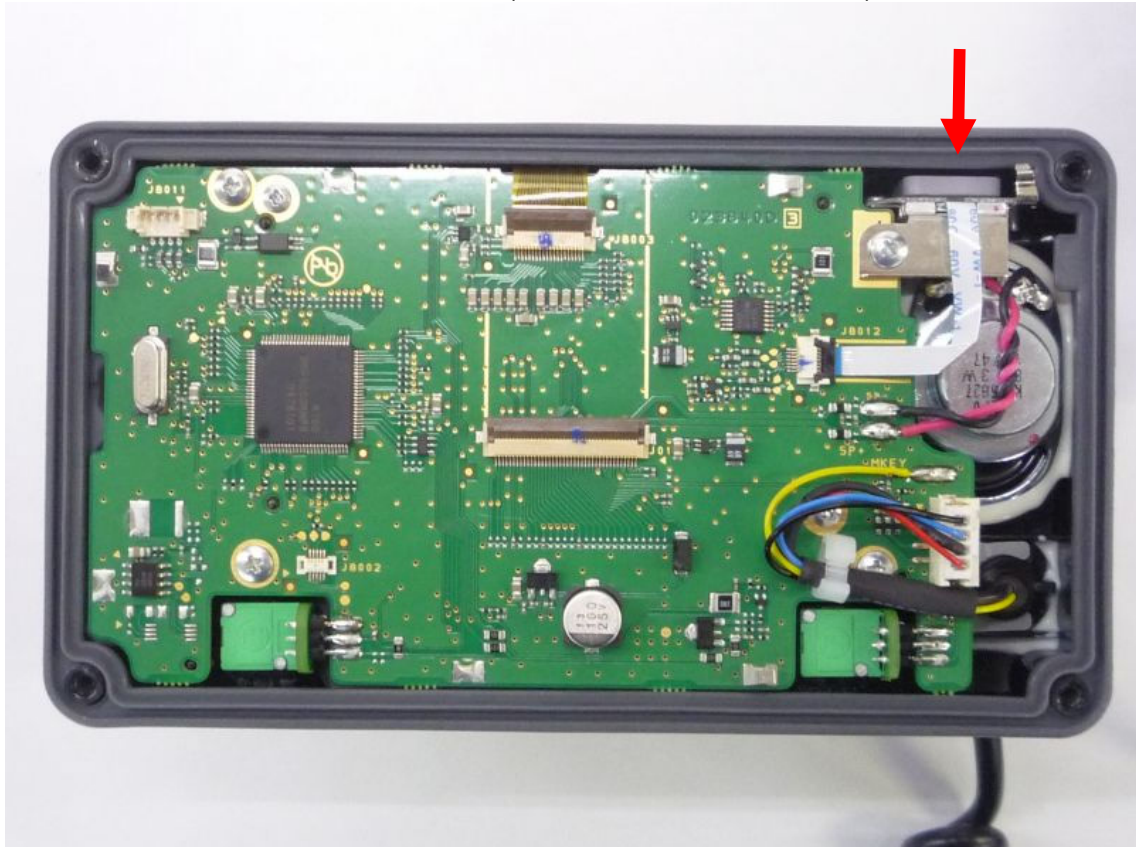
Back of Front Panel (GX1700 old GPS-UNIT Ver.)
