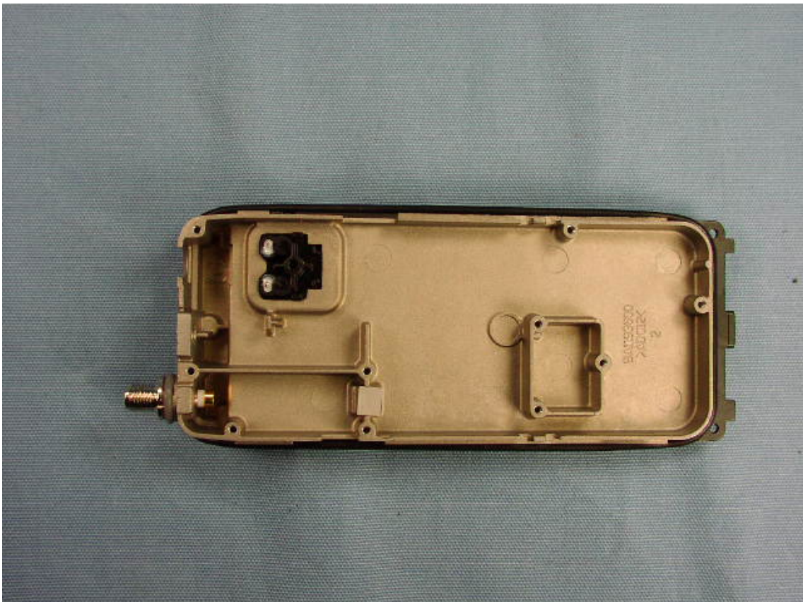
View of chassis (Removed Main Unit)
