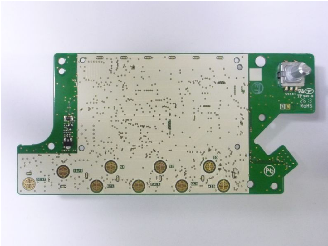
Side-A of CNTL-UNIT without LCD (GX2150)
