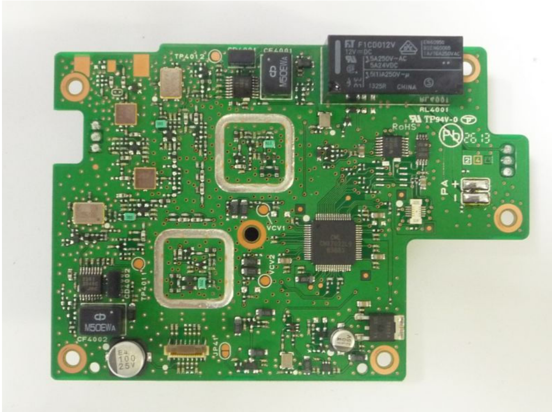
Side-A of AIS-UNIT without shield cases
