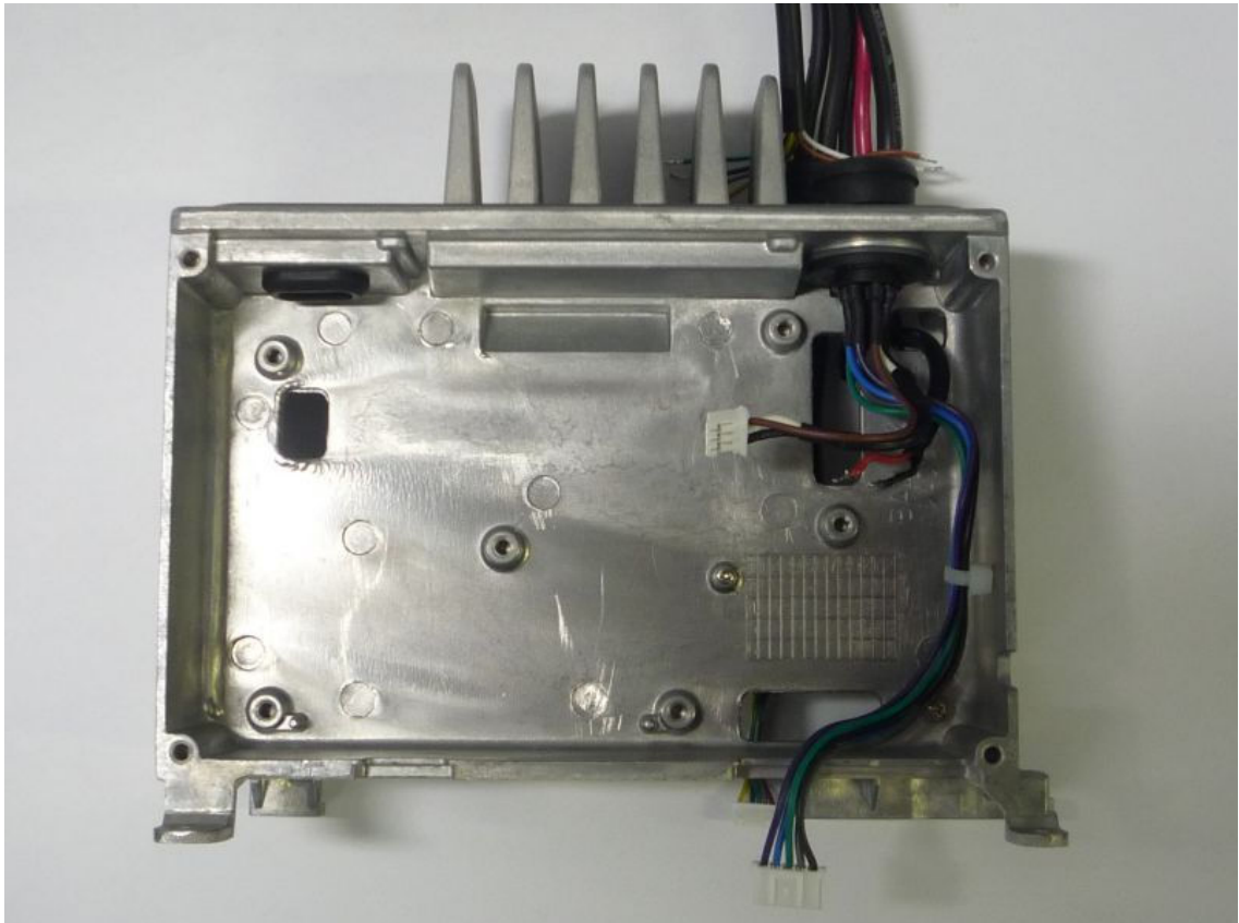
Inside of Chassis (Bottom view)
