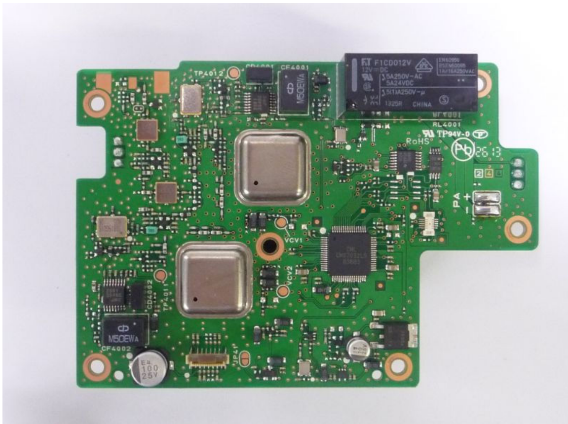
Side-A of AIS-UNIT with shield cases
