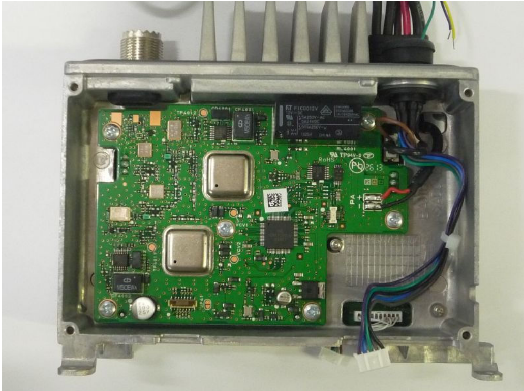
Chassis and AIS-Unit (Removed Front-Panel)
