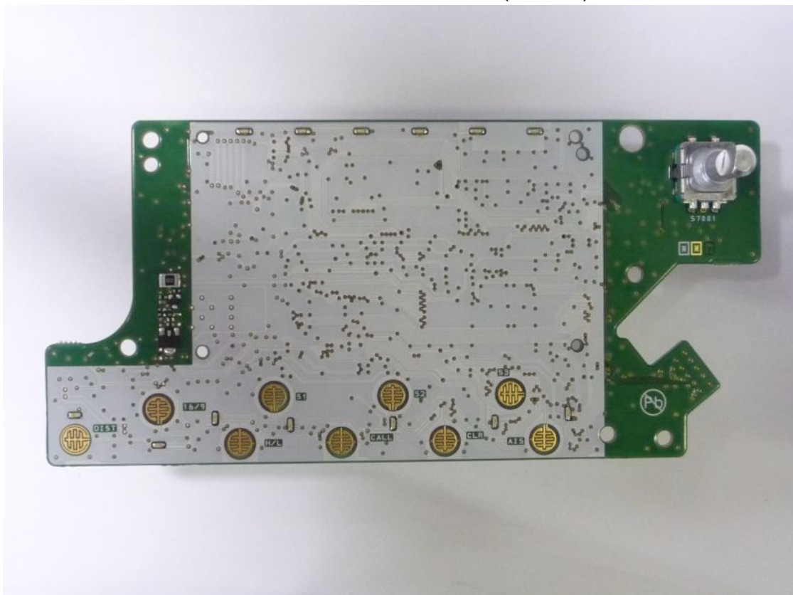
Side-A of CNTL-2 UNIT without LCD (GX2200)
