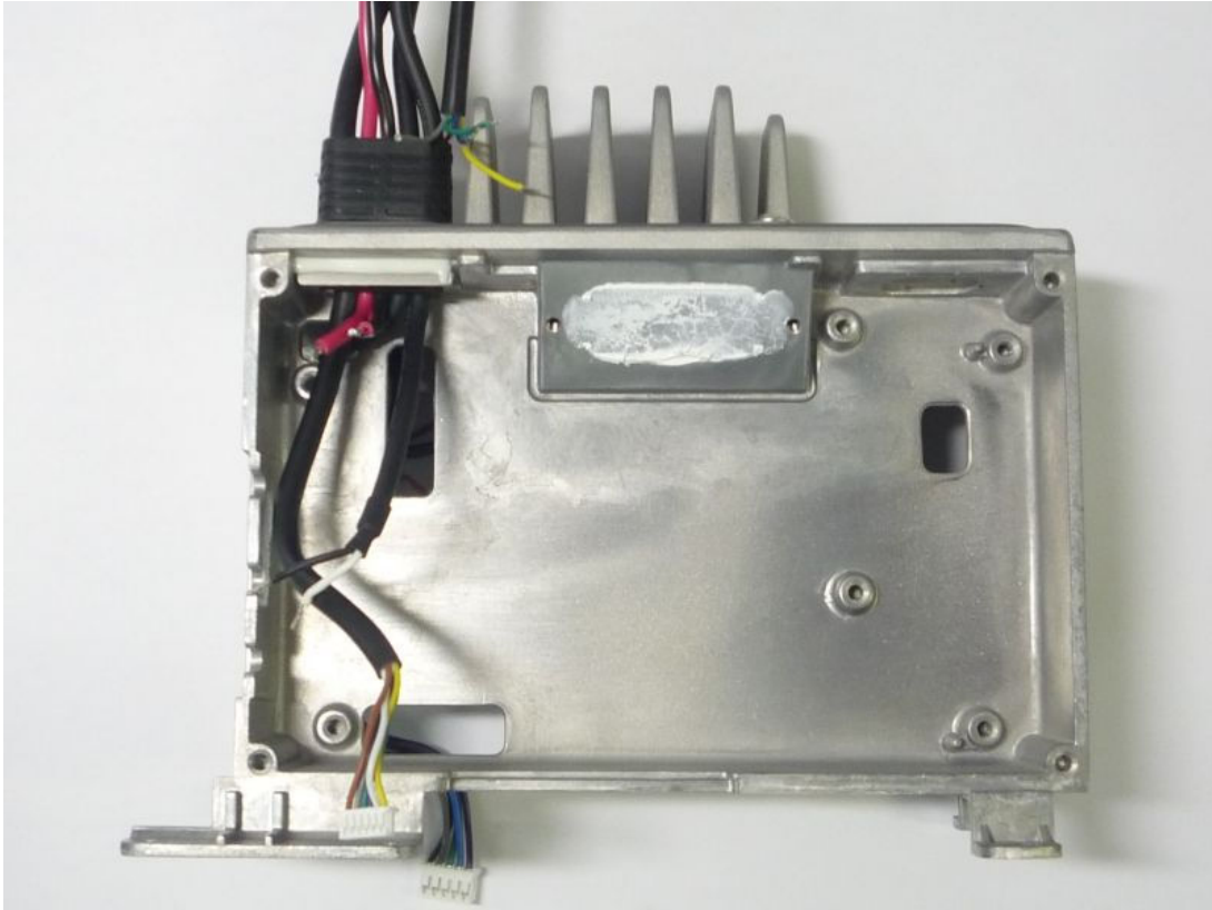
Inside of Chassis (Top view)
