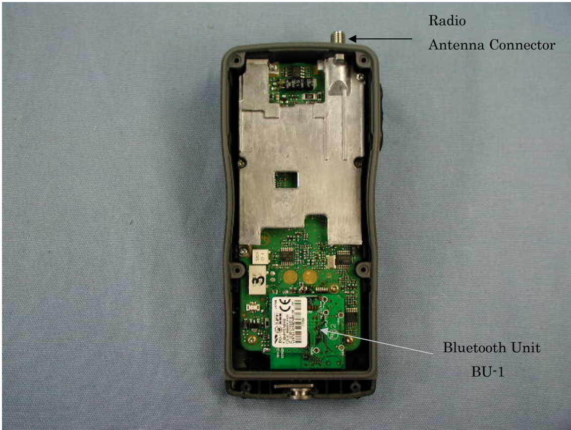
Removed Rear Panel with BU-1
