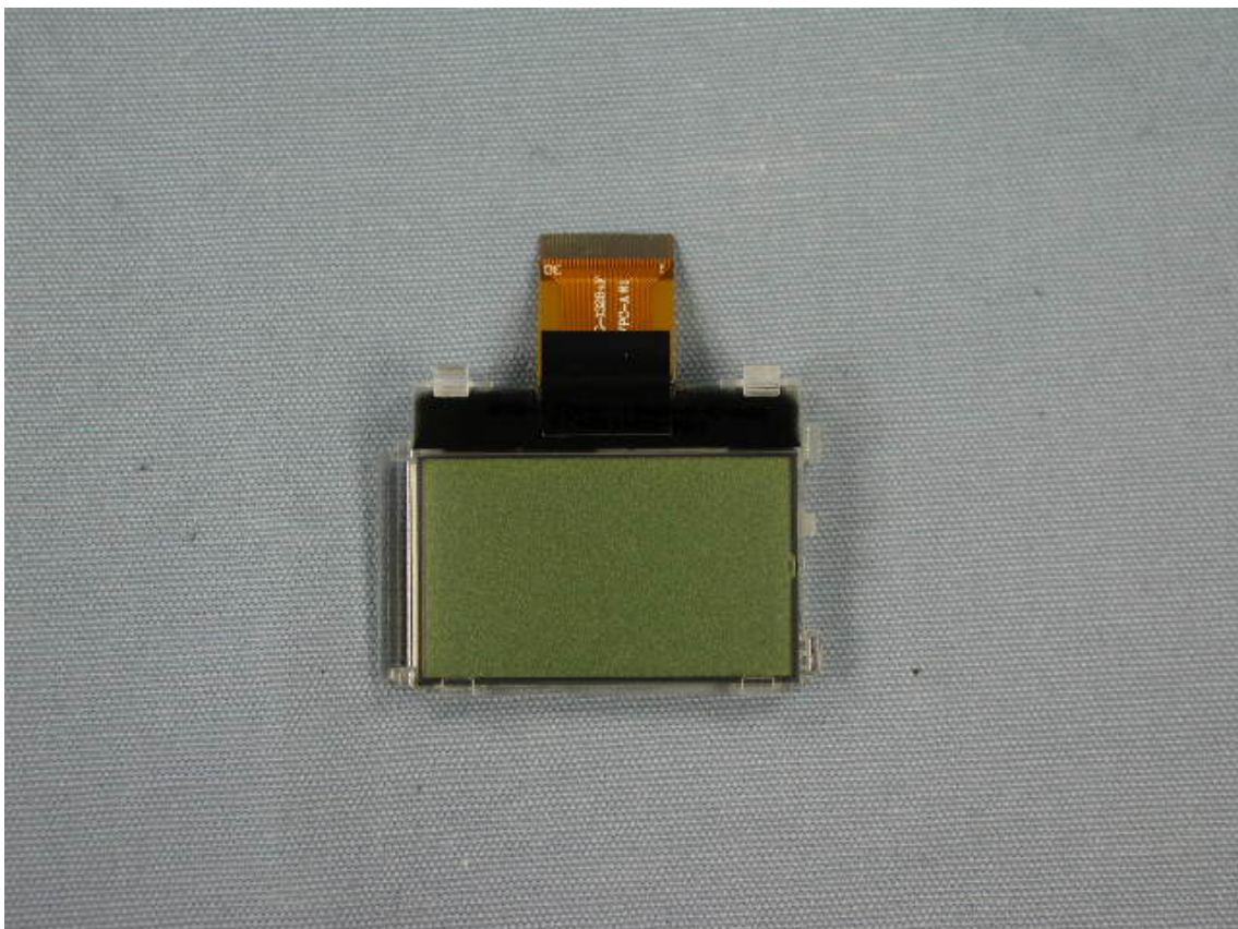
LCD (Front)
