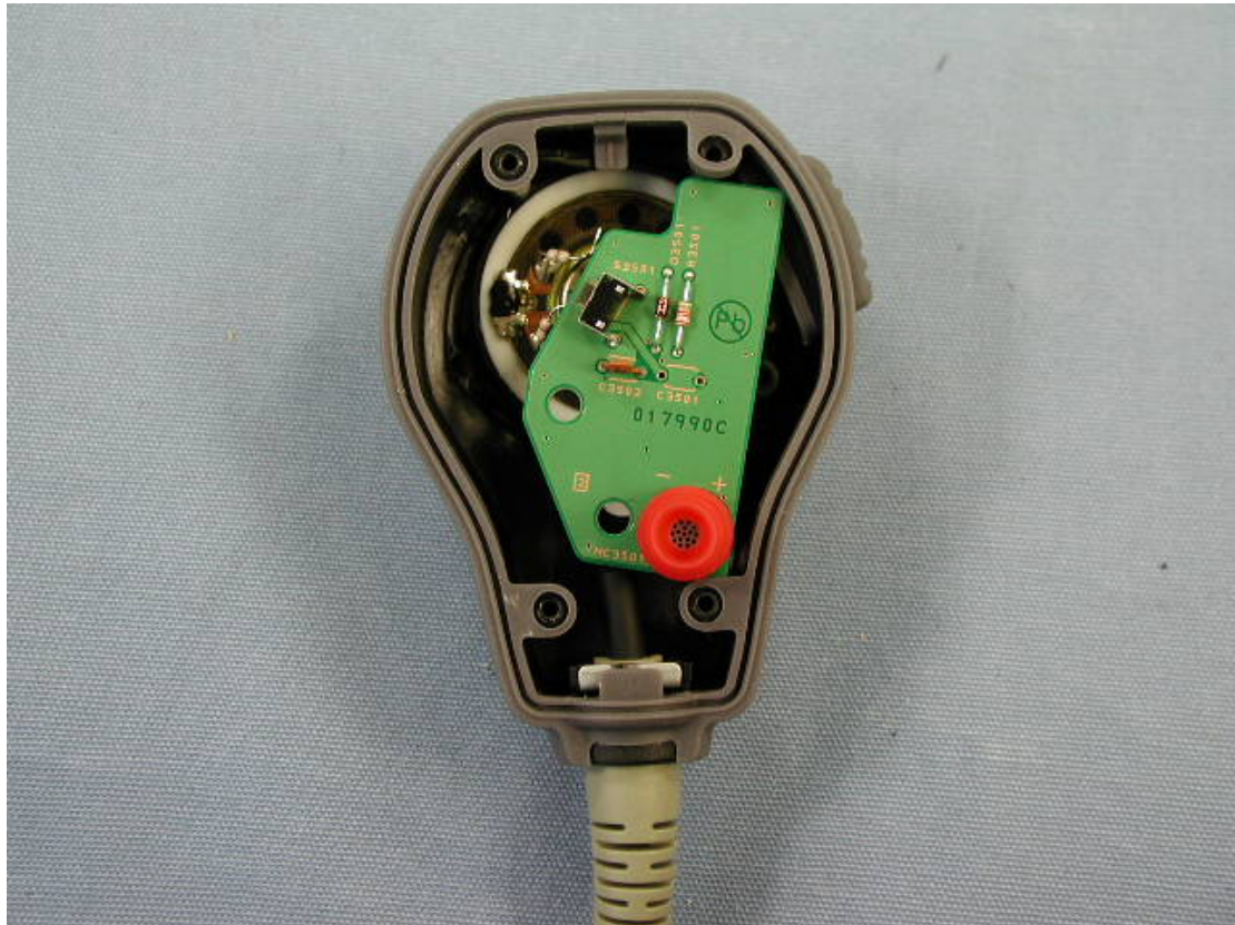
Inside of MH-73A4B (side B)
