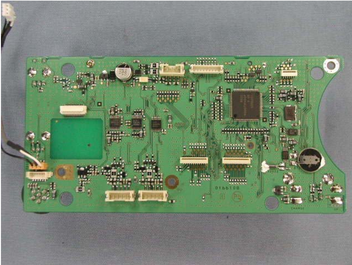
Side-B of CNTL-1-UNIT (GX5000S)
