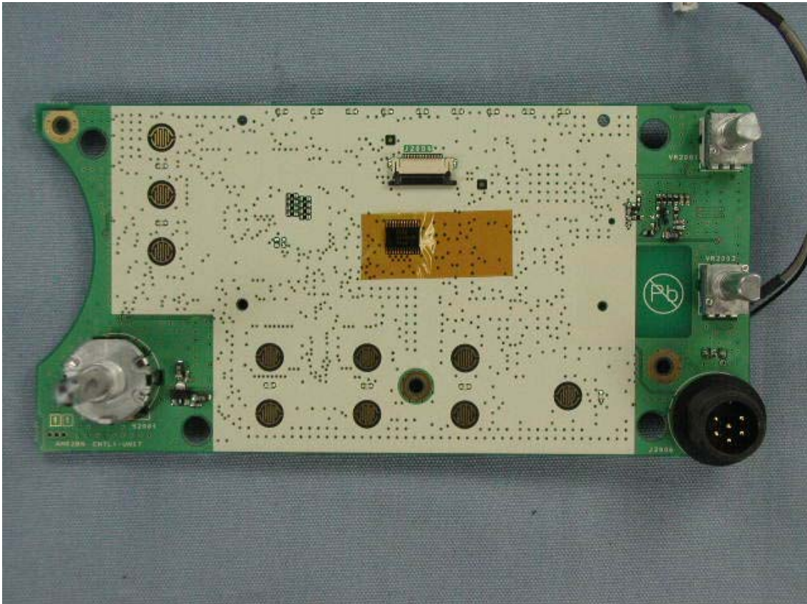
Side-A of CNTL-1-UNIT without LCD (GX5000S)
