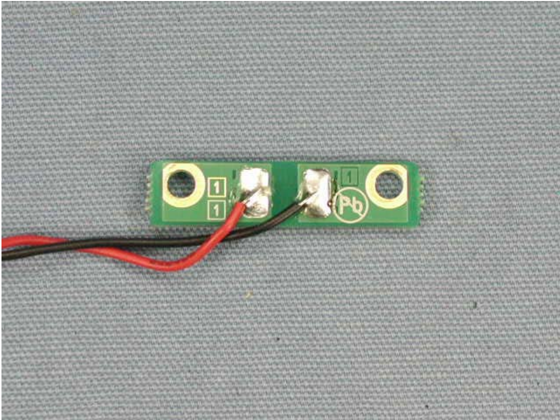
Side-A of TERMINAL-UNIT (GX5000S)/TERMINA-2-UNIT (GX5500S)
