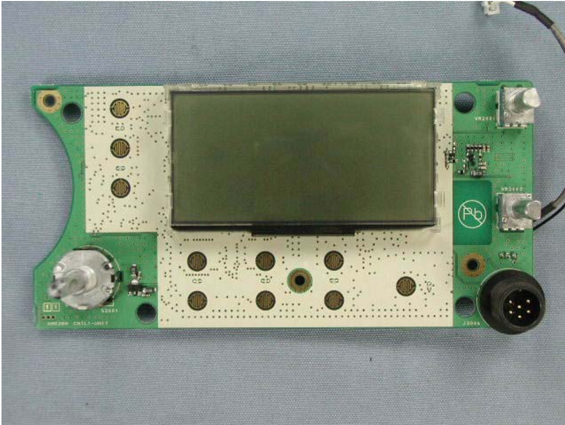
Side-A of CNTL-1-UNIT with LCD (GX5000S)
