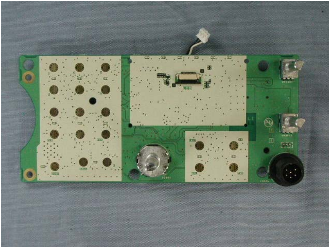
Side-A of CNTL-2-UNIT without LCD (GX5500S)
