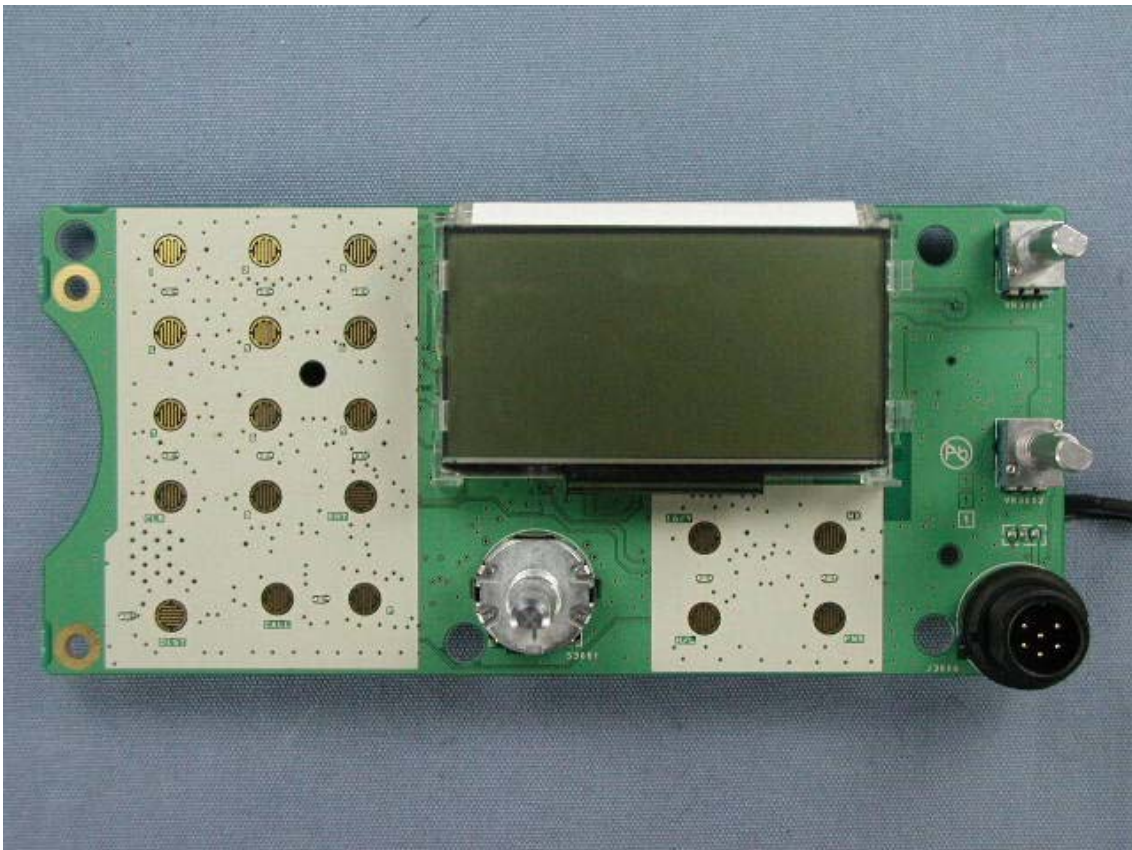
Side-A of CNTL-2-UNIT with LCD (GX5500S)
