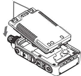
Battery Latches
