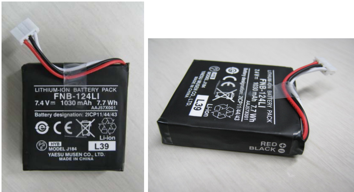
Fig.5-1 FNB-124LI (Angle-1 & Angle-2)
