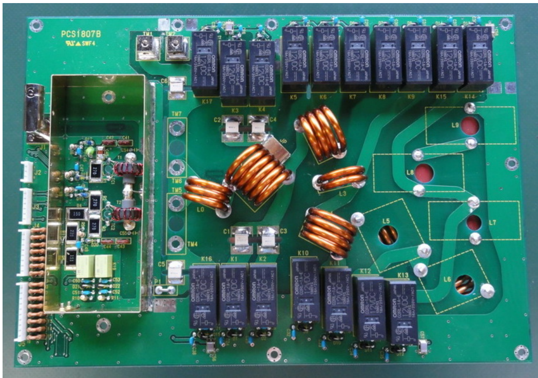
View of DET/NETWORK UNIT without Shield Cover (Side-A)
