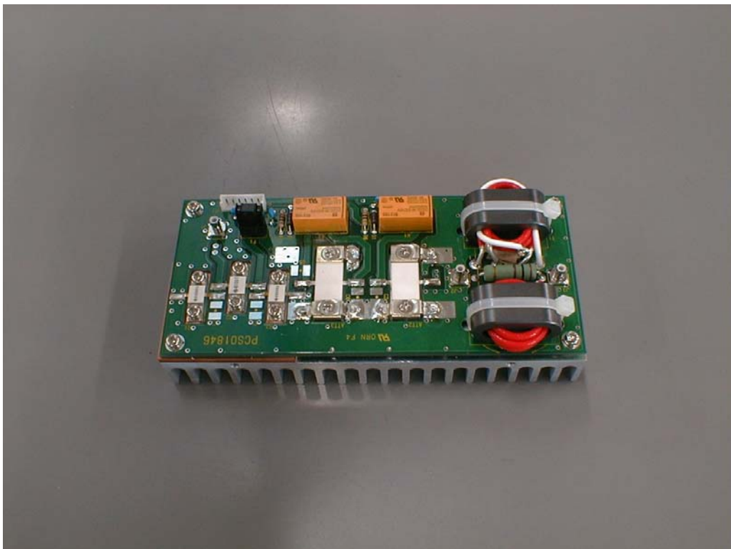
View of ATT UNIT with heat sink (Side-A)
