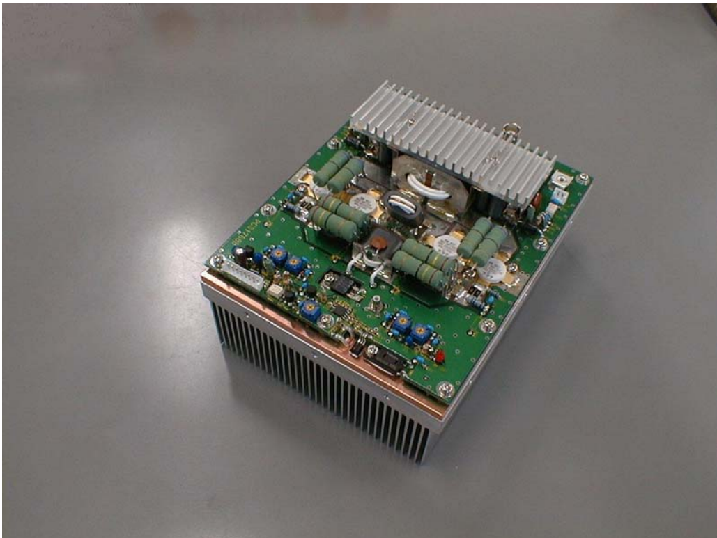
View of PA UNIT with Heat sink (Side-A)
