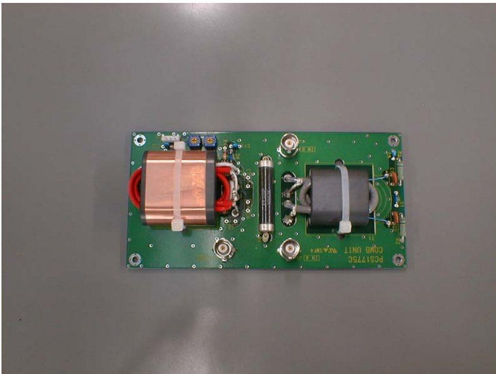
View of COMB UNIT (Side-A)
