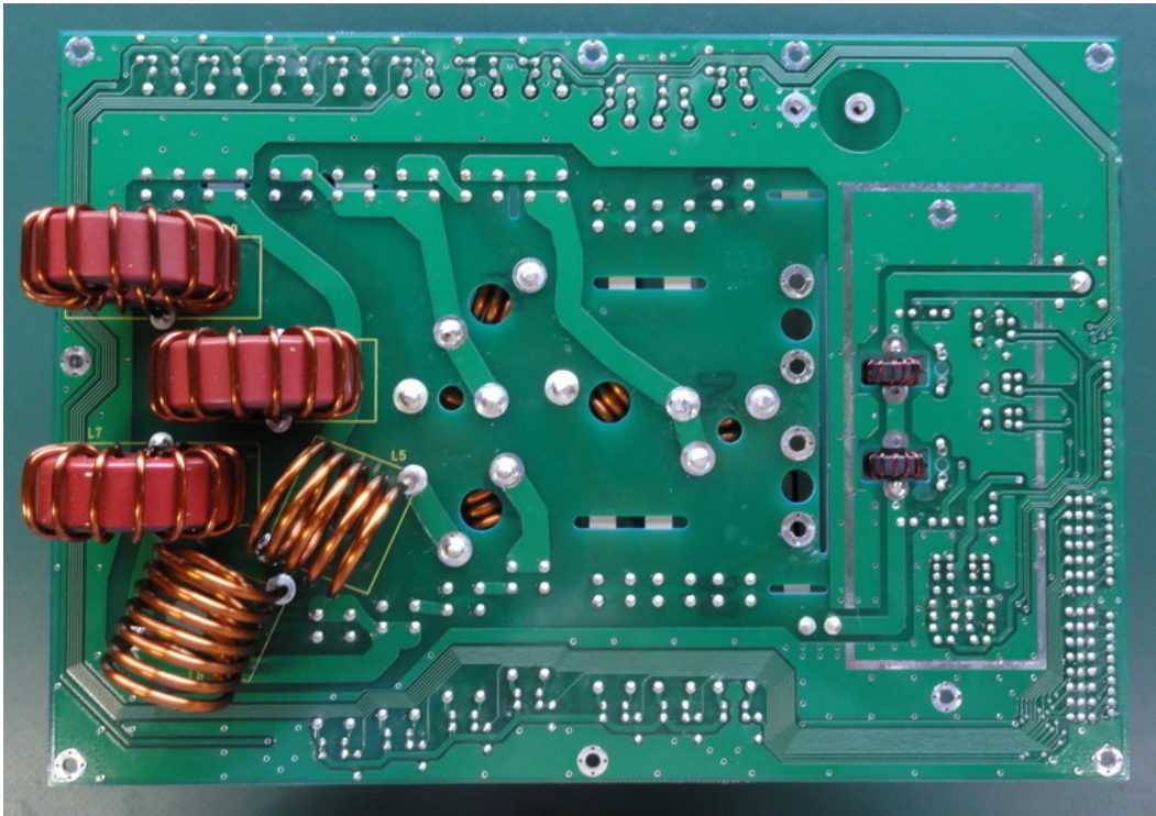
View of DET/NETWORK UNIT (Side-B)
