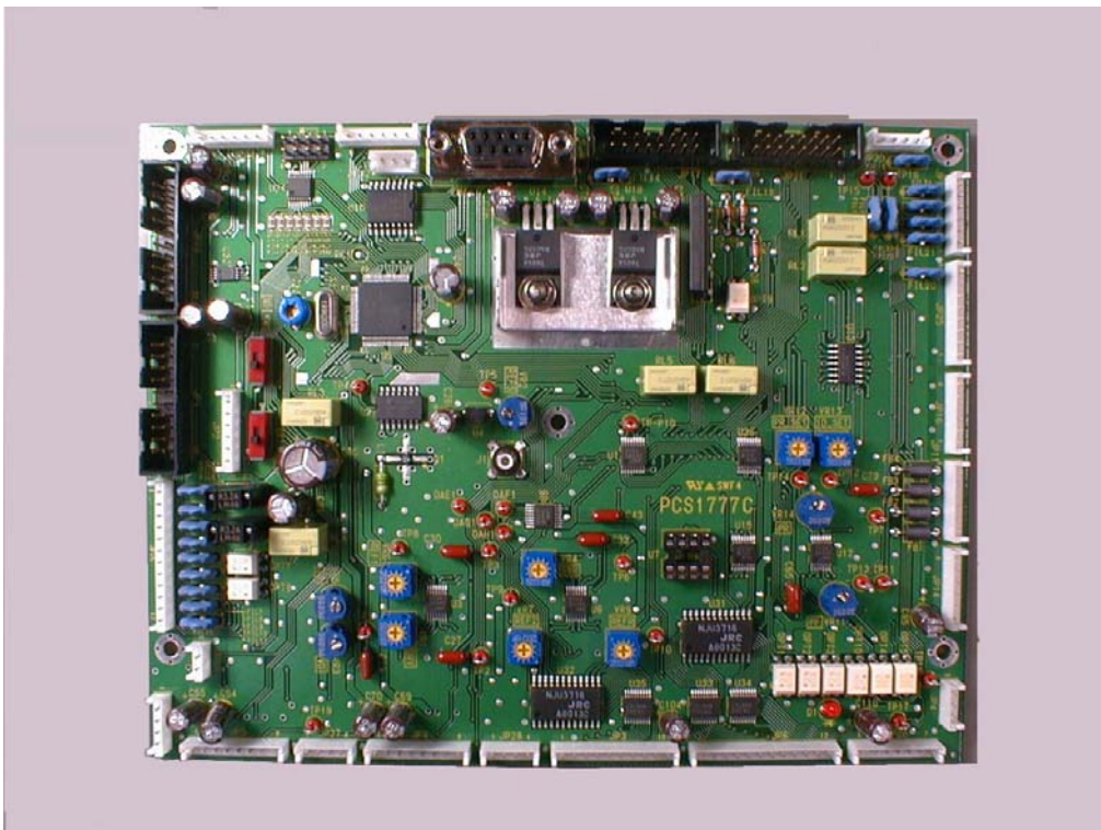
View of VL_CONT UNIT (Side-A)
