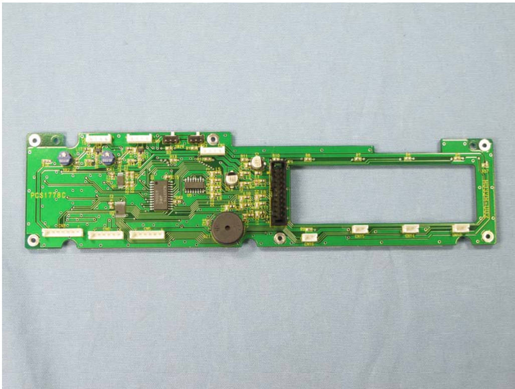
View of DISPLAY-UNIT (Side-A)
