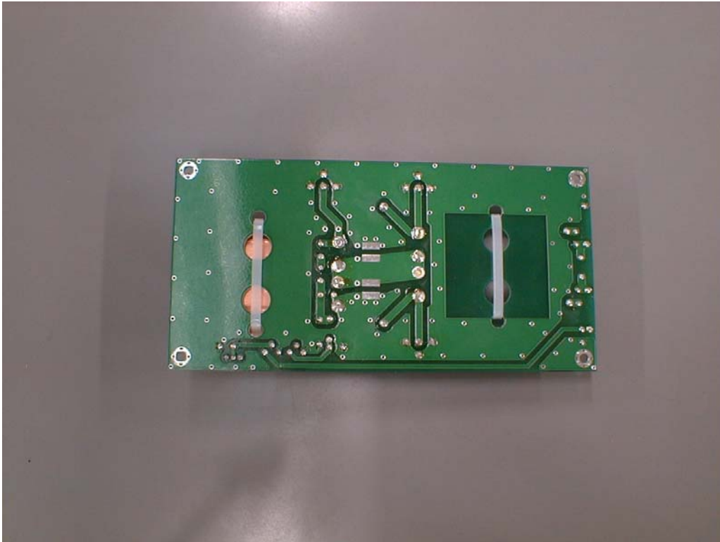
View of COMB UNIT (Side-B)
