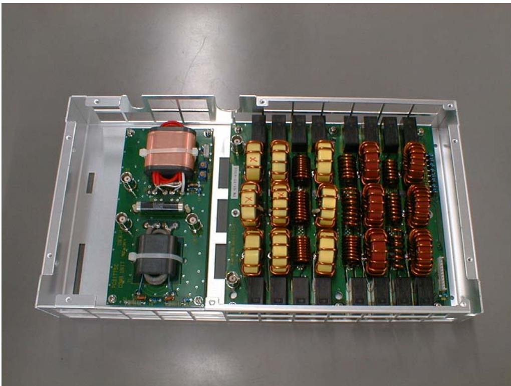
View of LPF / COMB UNIT with Shield Case
