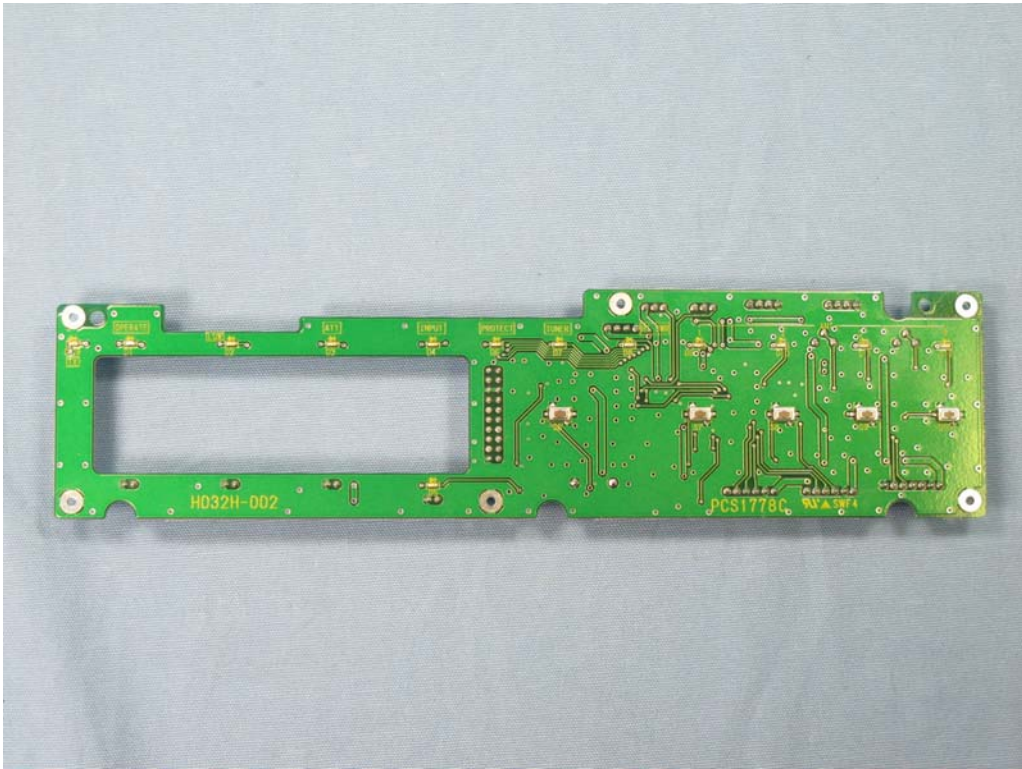
View of DISPLAY-UNIT (Side-B)
