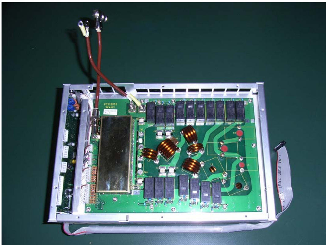
View of NETWORK / TUNNER CPU UNIT with Shield Case (Side-A)
