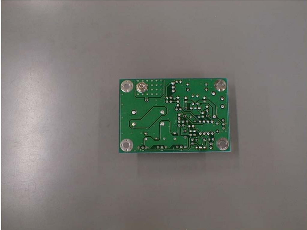
View of FAN_CTRL UNIT (Side-B)
