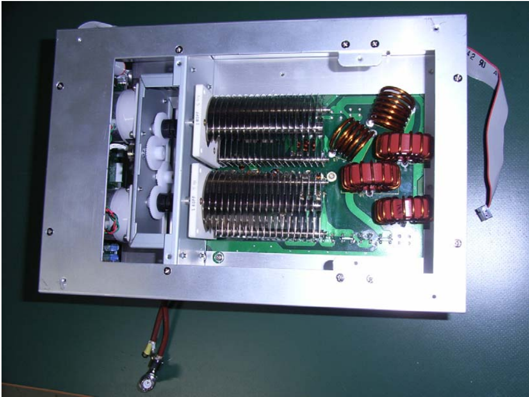
View of NETWORK / TUNNER CPU UNIT with Shield Case (Side-B)
