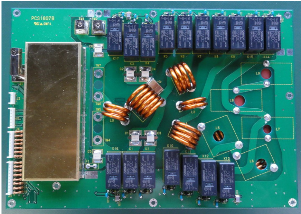
View of DET/NETWORK UNIT (Side-A)
