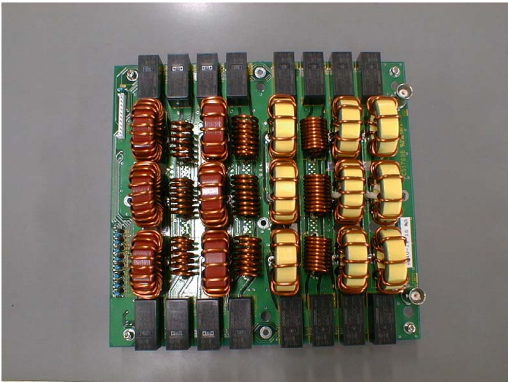
View of LPF UNIT (Side-A)
