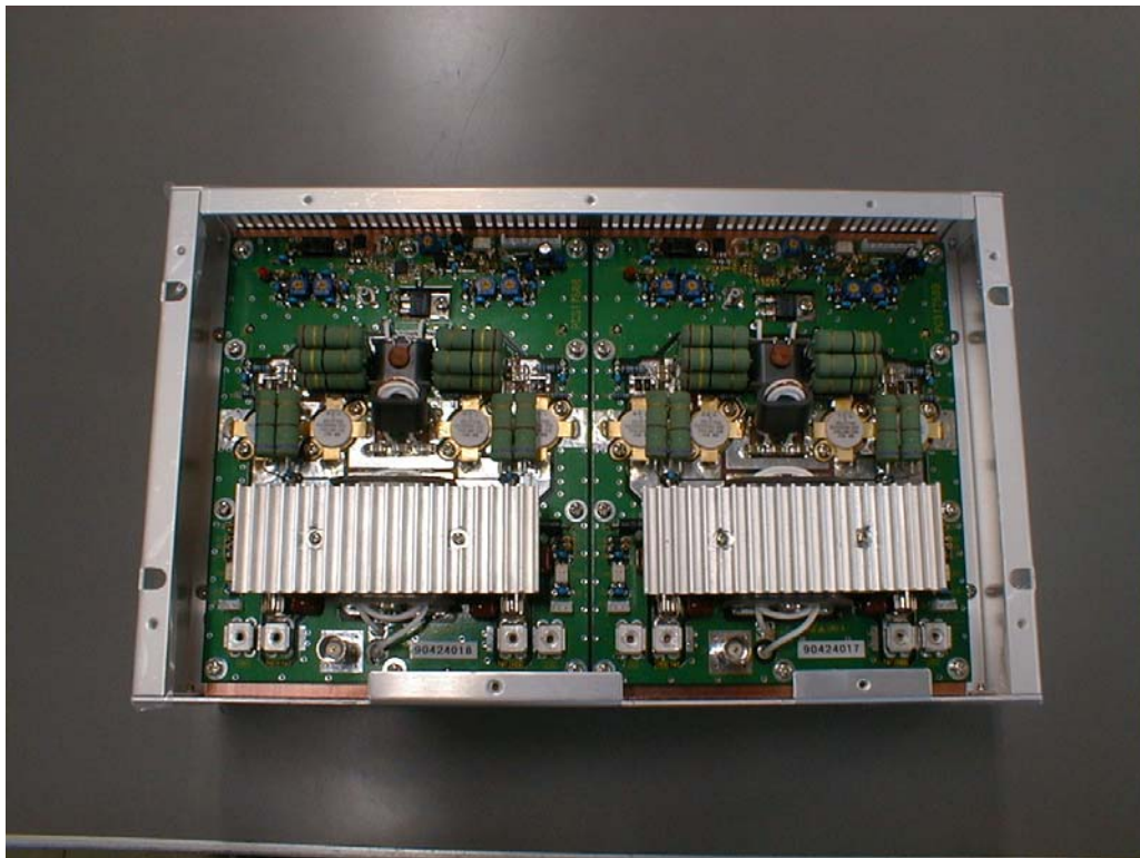
View of PA UNIT Block
