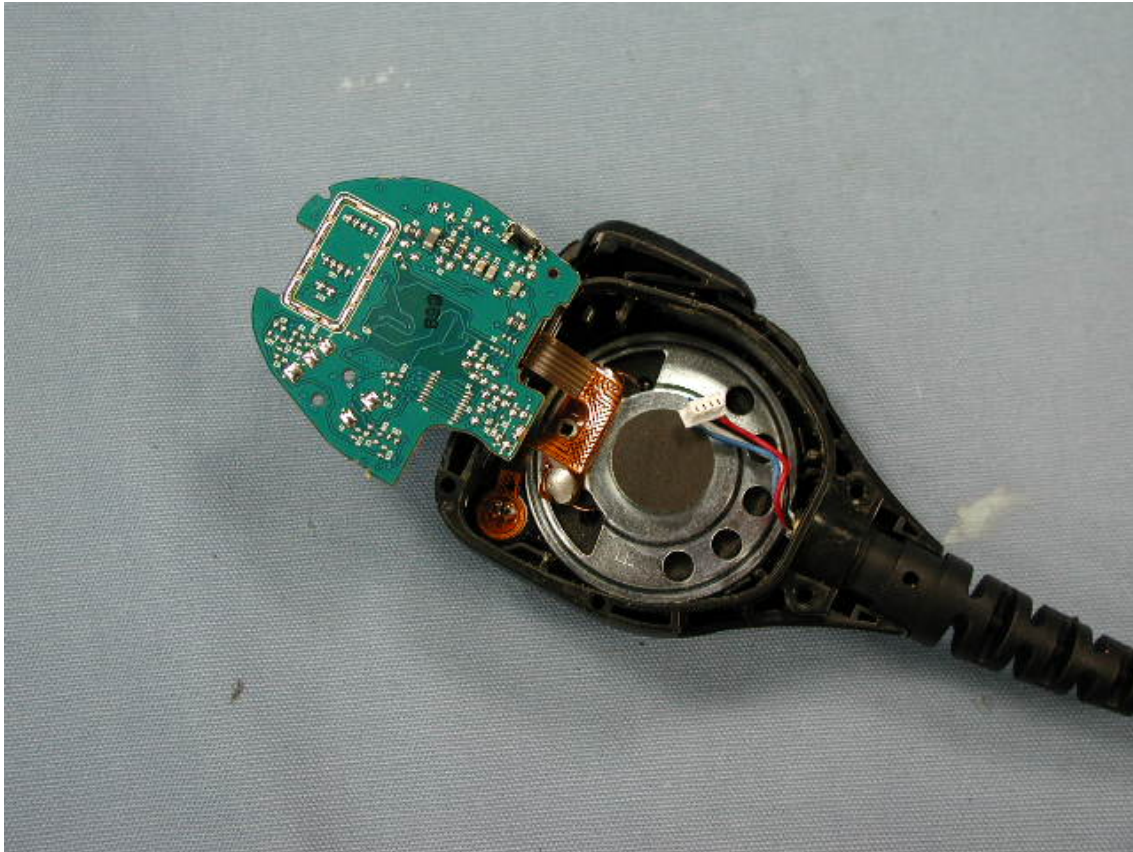
Inside of Microphone PCB Side-B
