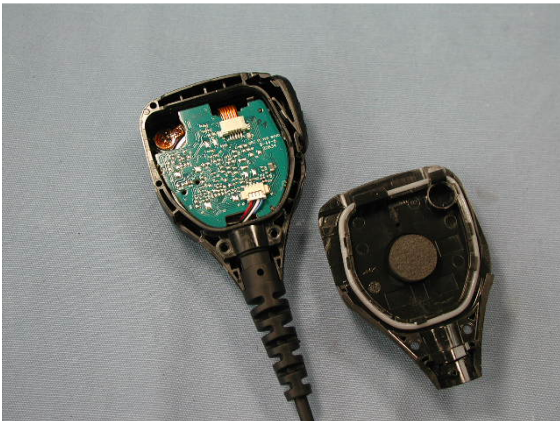
Inside of Microphone PCB Side-A
