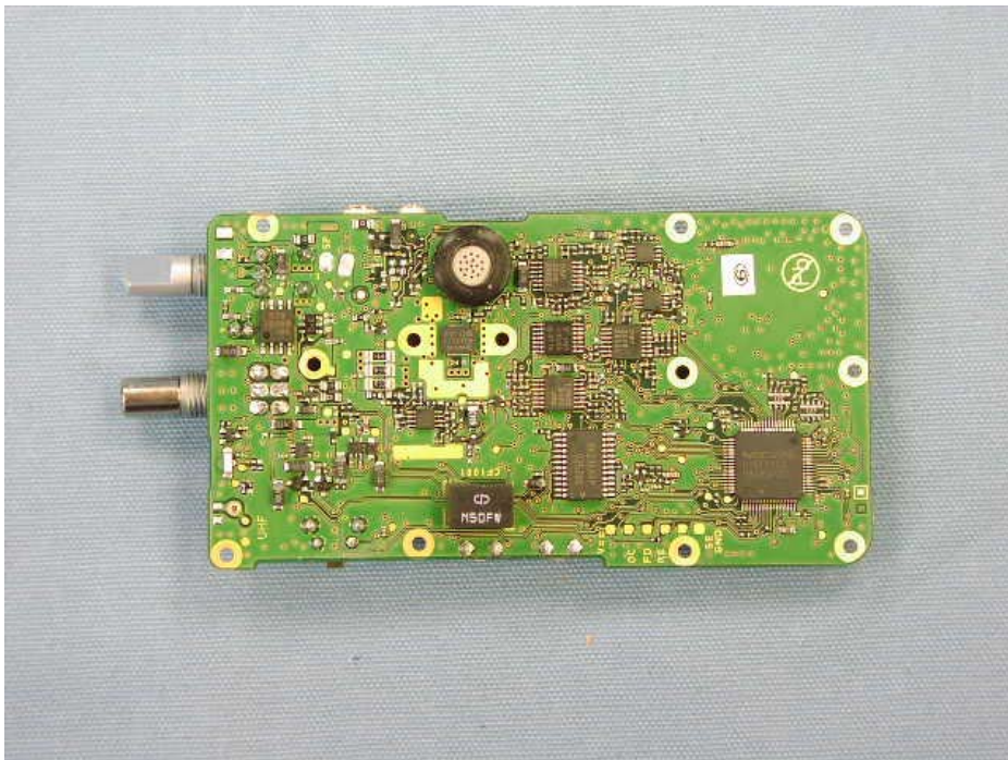
BC95 Side-A of Main-Unit
