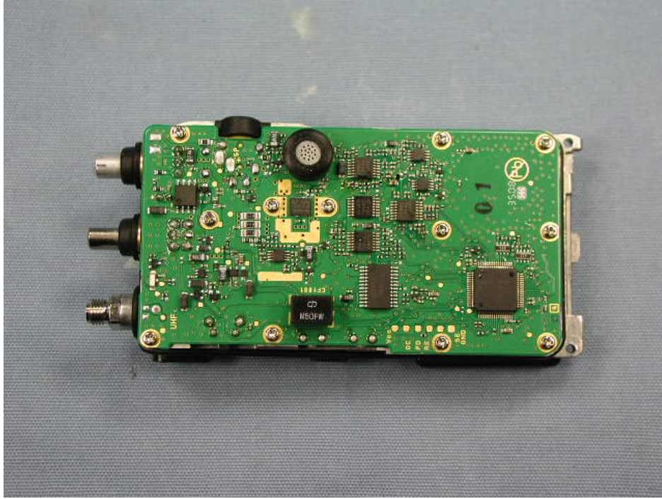
VX-231-AG6B-5 Side-A of Main-Unit
