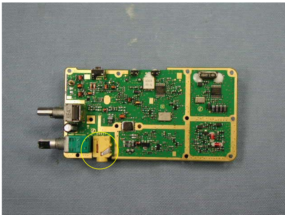
VX-231-AG6B-5 Side-B of Main-Unit
