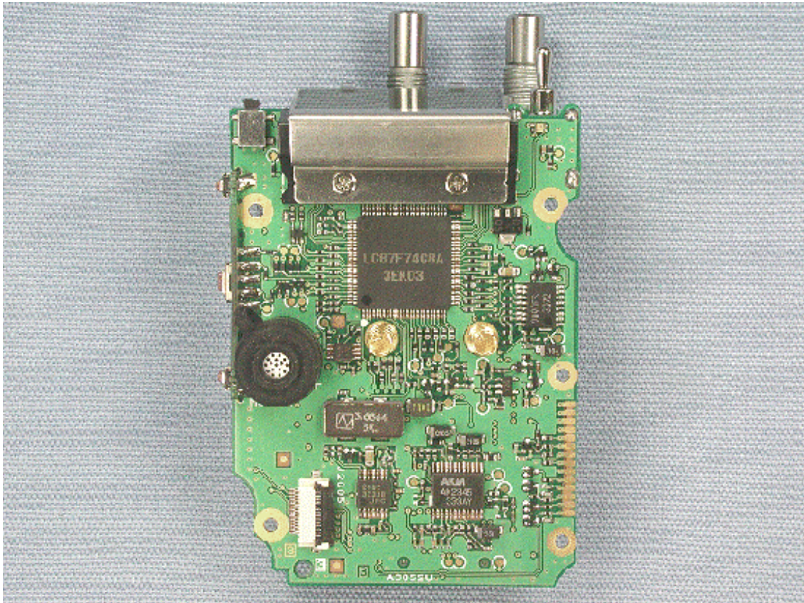
CNTL-UNIT with LCD/PTT-UNIT/VR-UNIT
