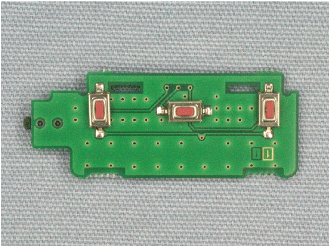
Side-A of PTT-UNIT
