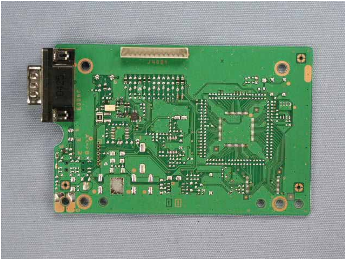
Side-A of GPS-INTERFACE-UNIT
