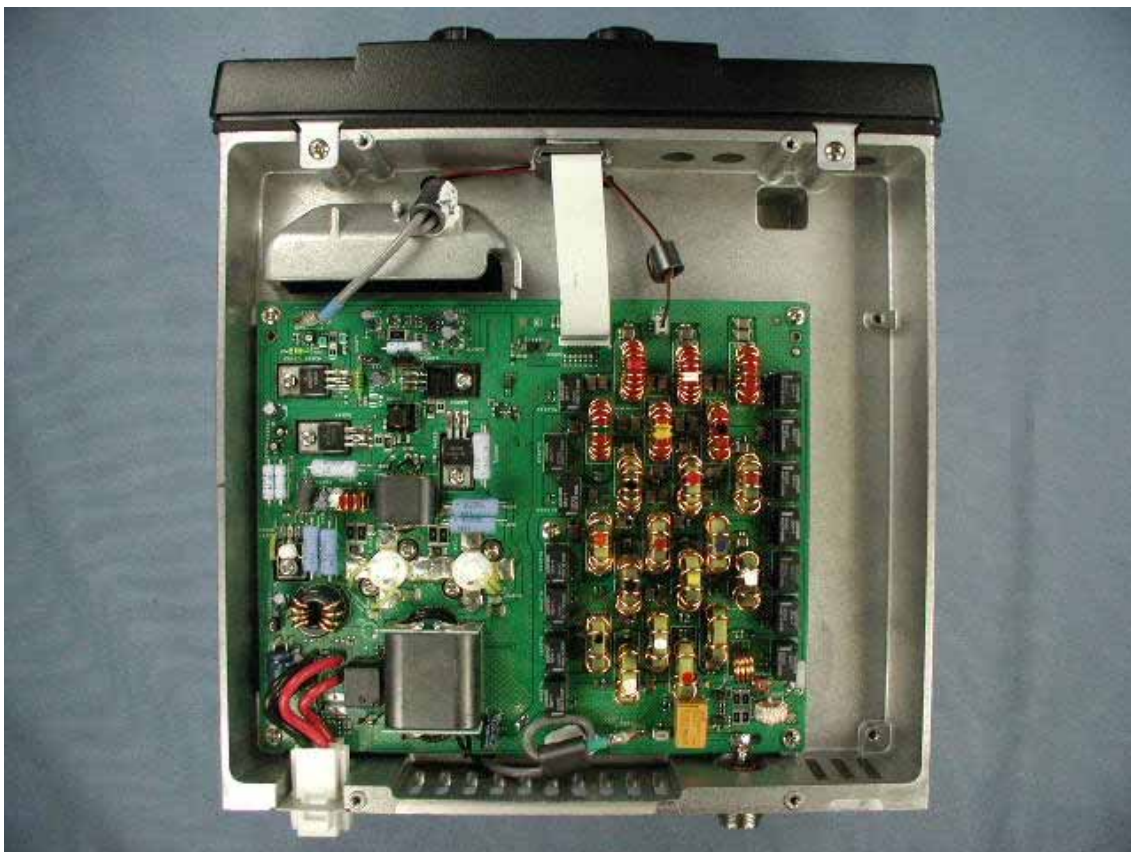
Top case opened
