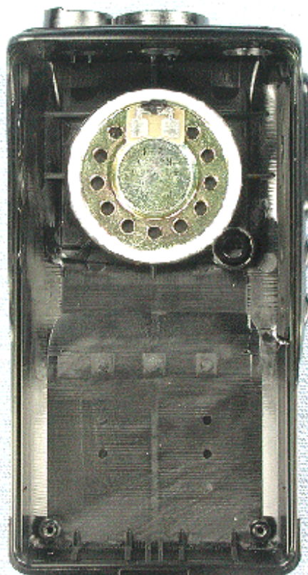
Inside of front panel (VX-414)
