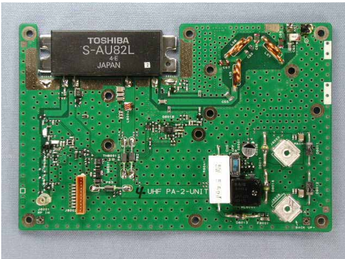
Side-B of PA-2-UNIT without shield case
