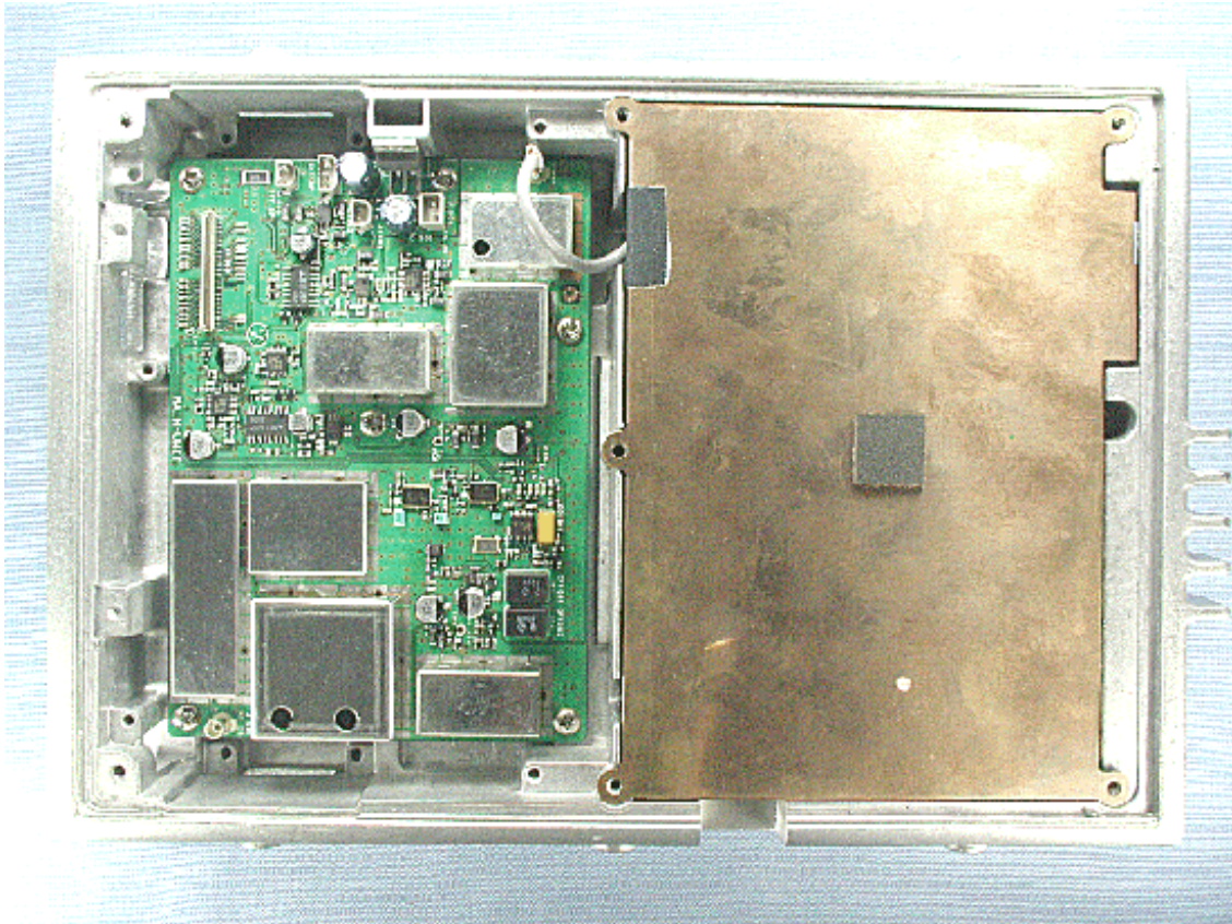
Inside of sub-chassis with shield cover
