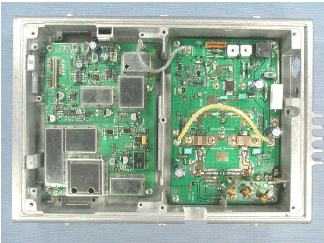
Inside of sub-chassis without shield cover
