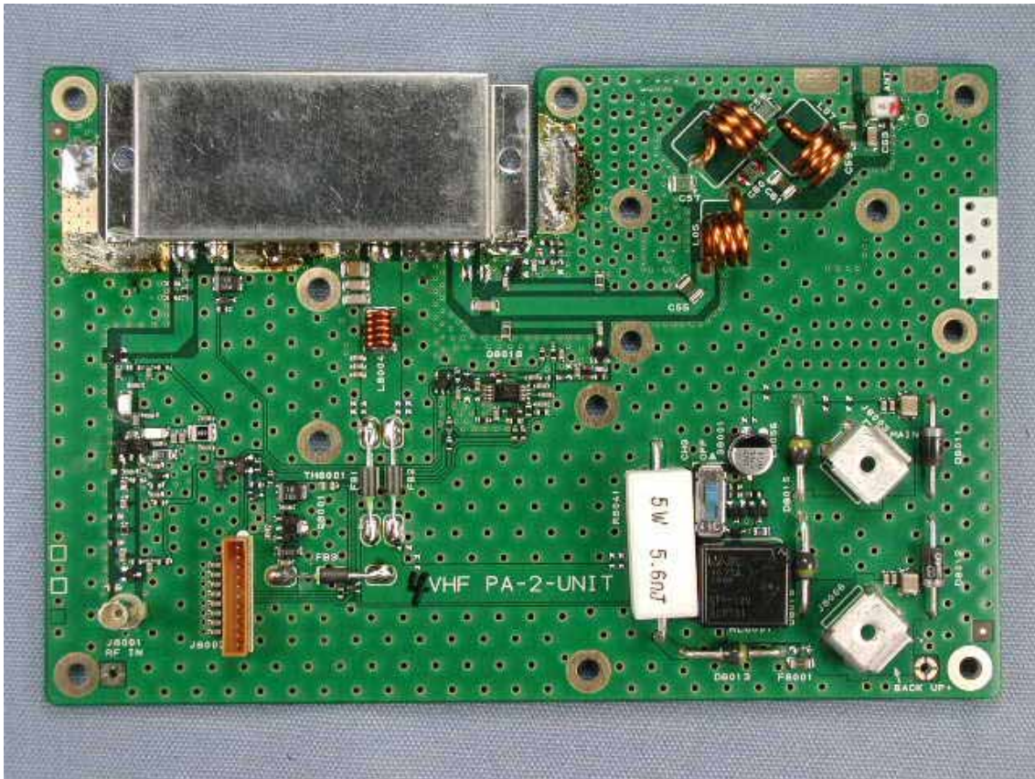
Side-A of PA-2-UNIT with shield case
