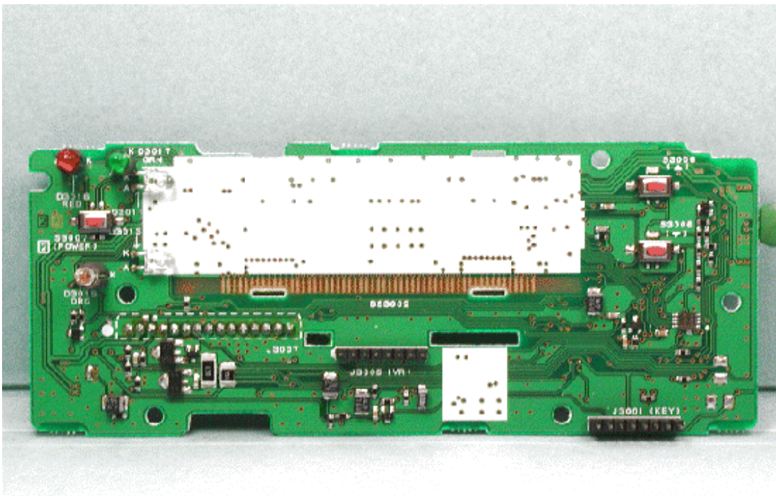
Side-A of DISPLAY-UNIT without LCD
