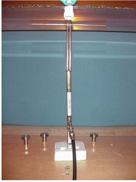
450MHz Dipole Setup
